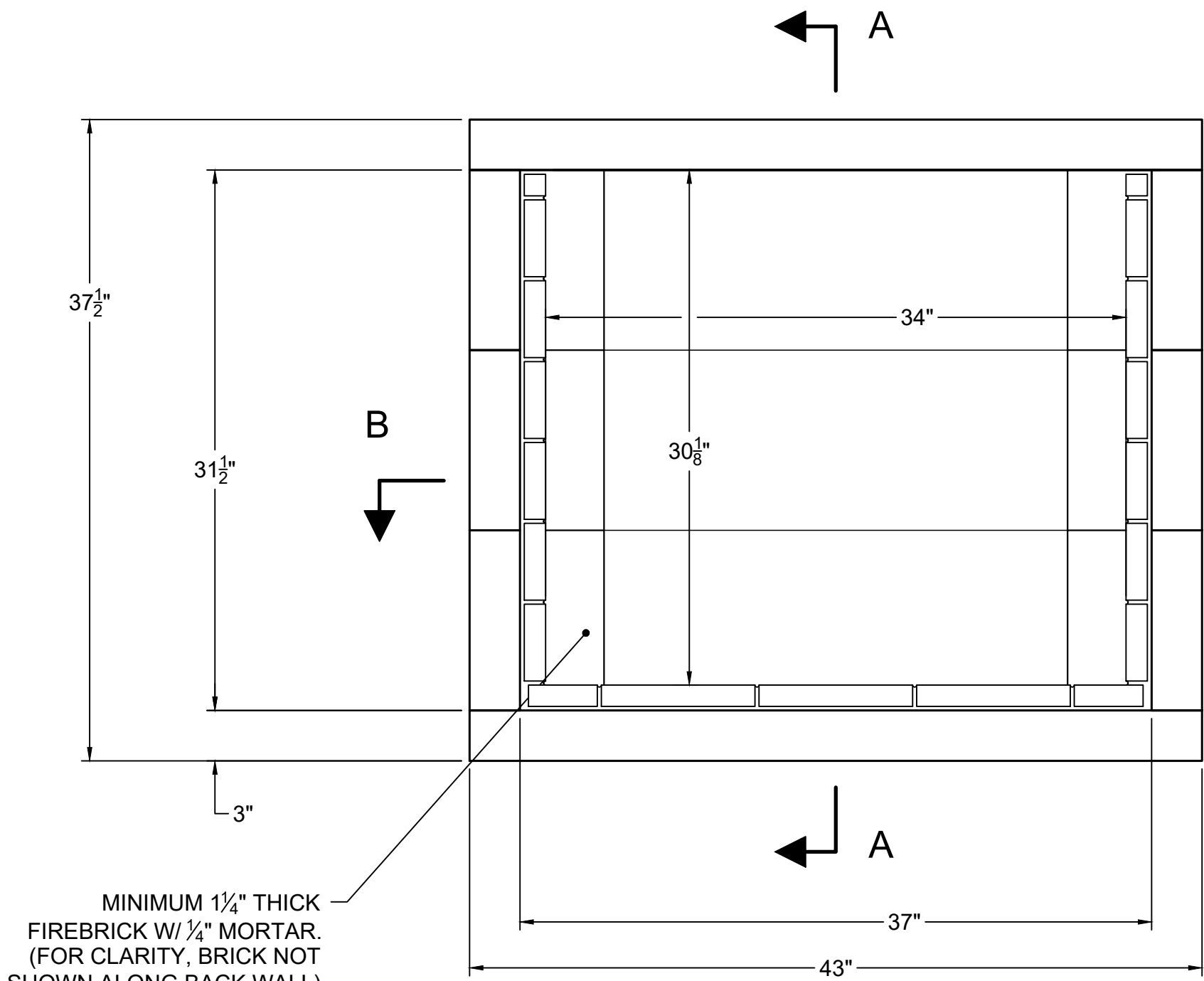
FRONT VIEW
