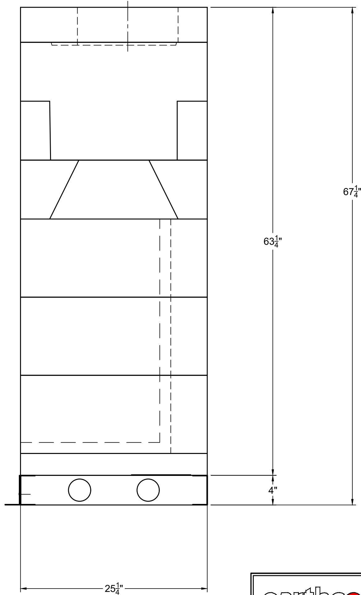
RIGHT-SIDE VIEW
