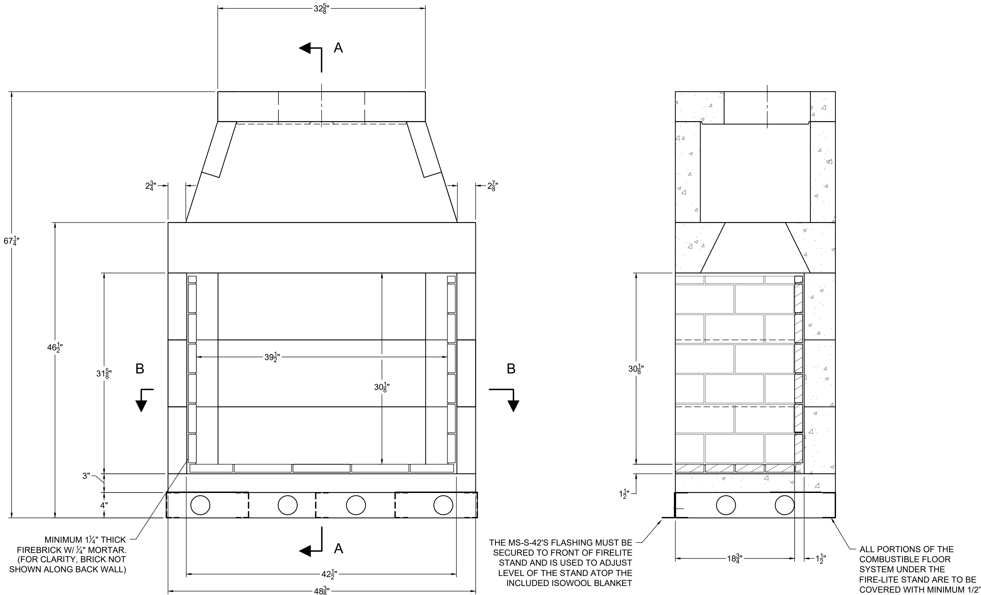
FRONT VIEW *MS-S-42 FLASHING NOT SHOWN IN VIEW*
