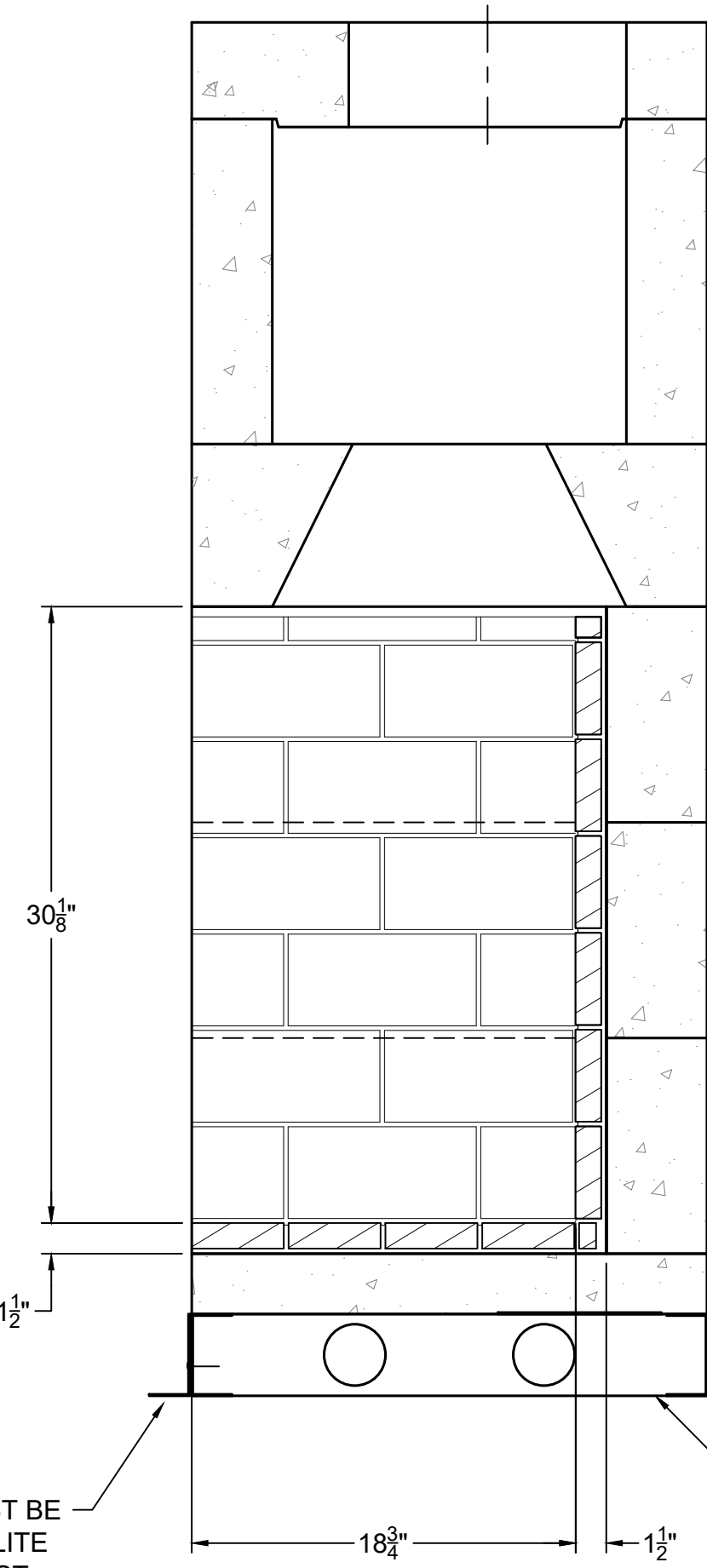
SECTION A-A VERTICAL FIREBRICK DETAIL
