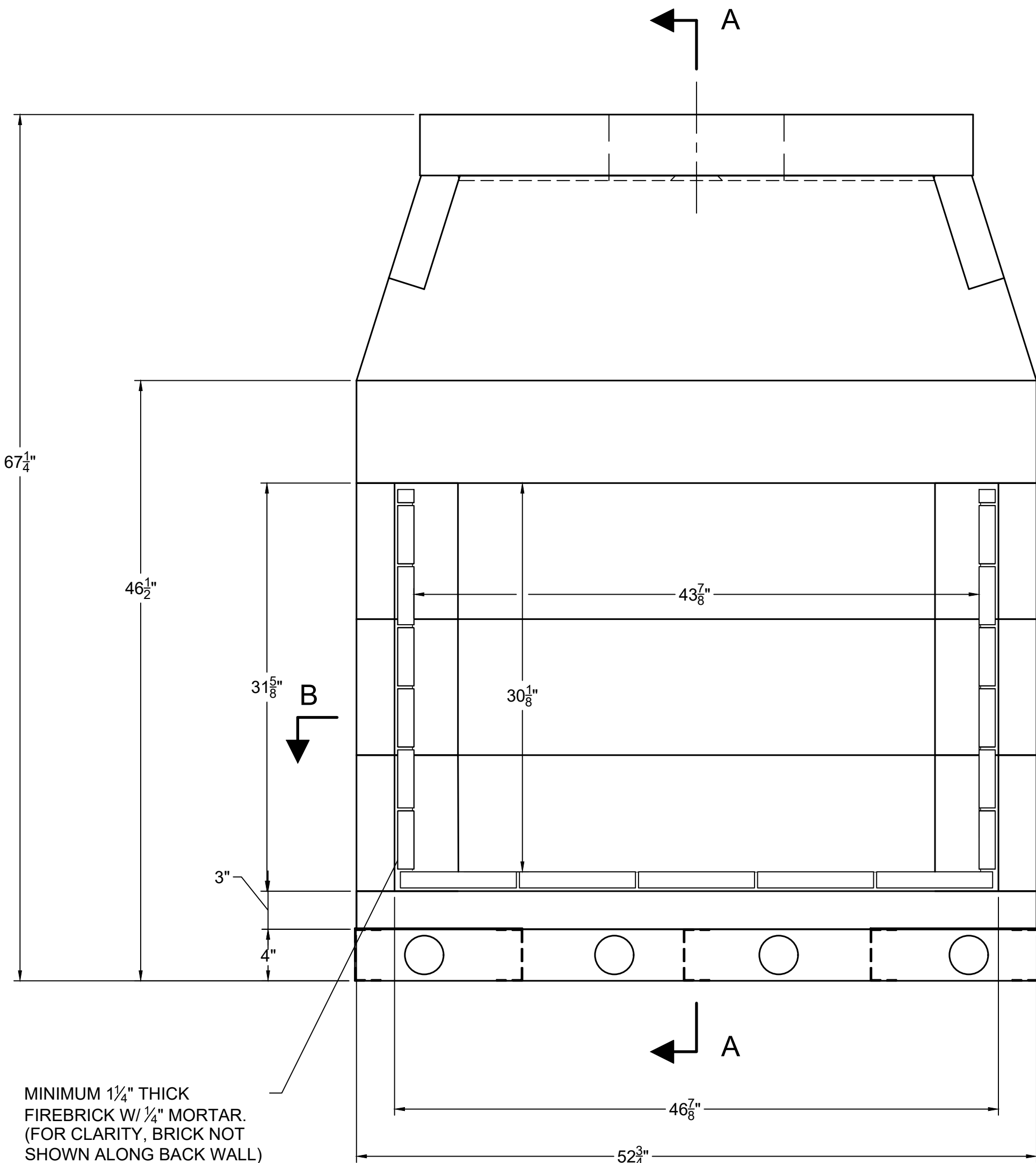
FRONT VIEW
