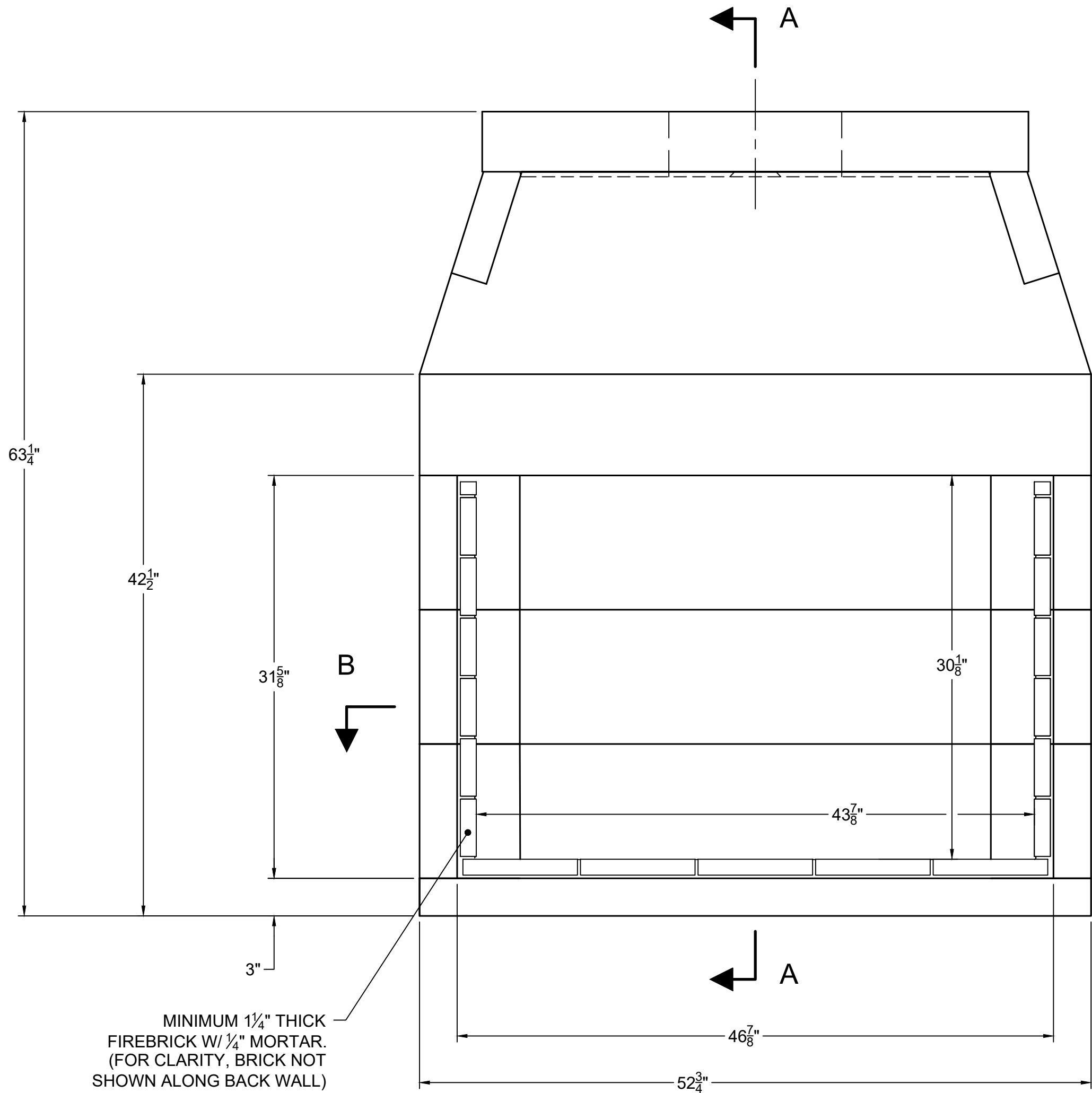
FRONT VIEW
