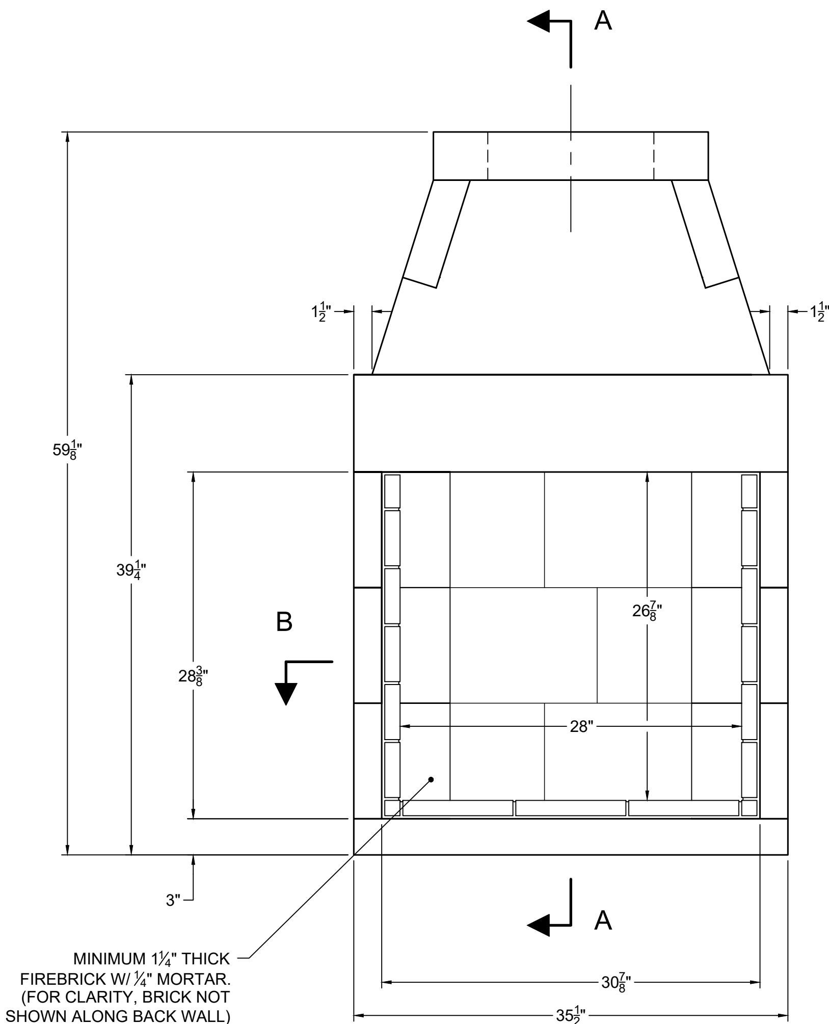
FRONT VIEW
