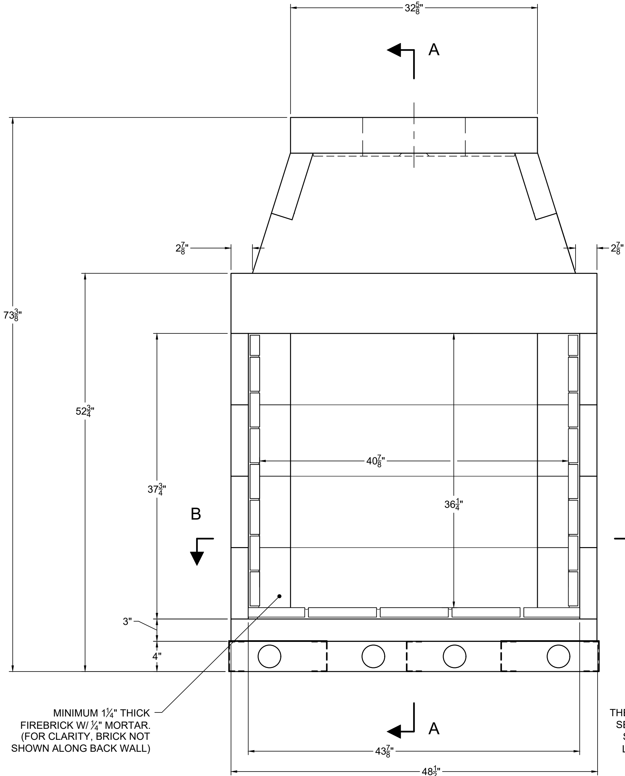
FRONT VIEW
