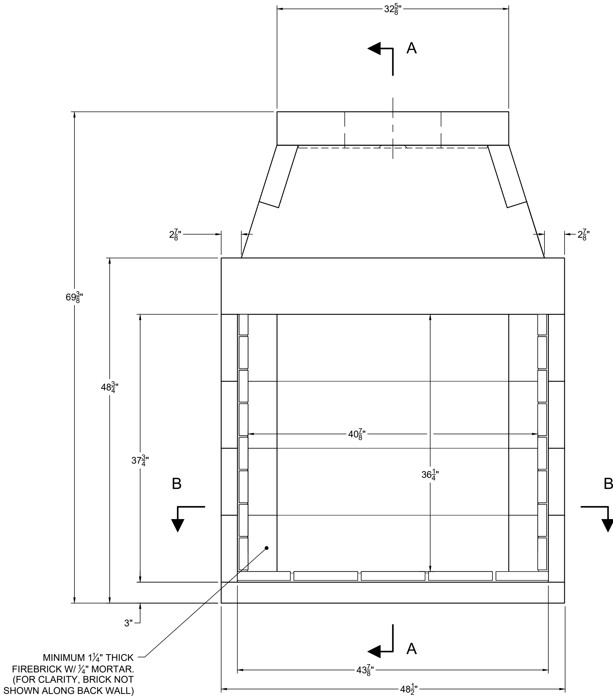
FRONT VIEW
