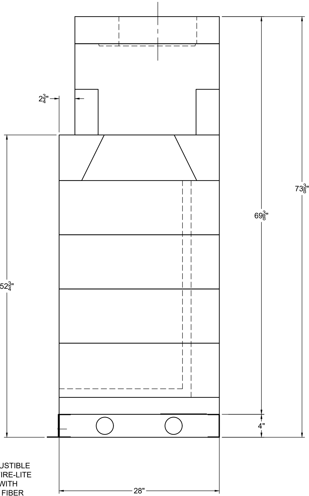
RIGHT-SIDE VIEW
