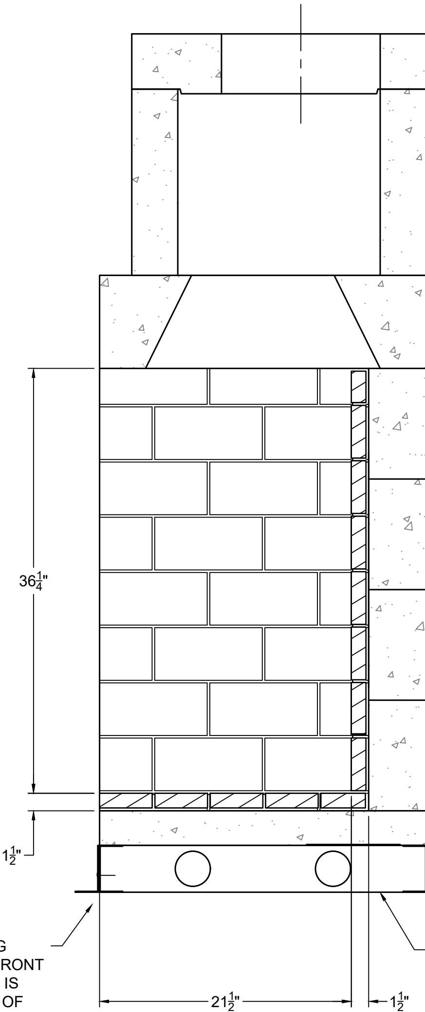
SECTION A-A VERTICAL FIREBRICK DETAIL
