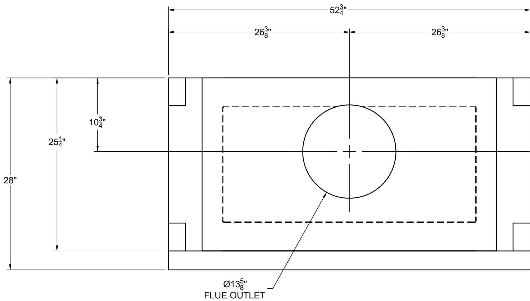
TOP VIEW
