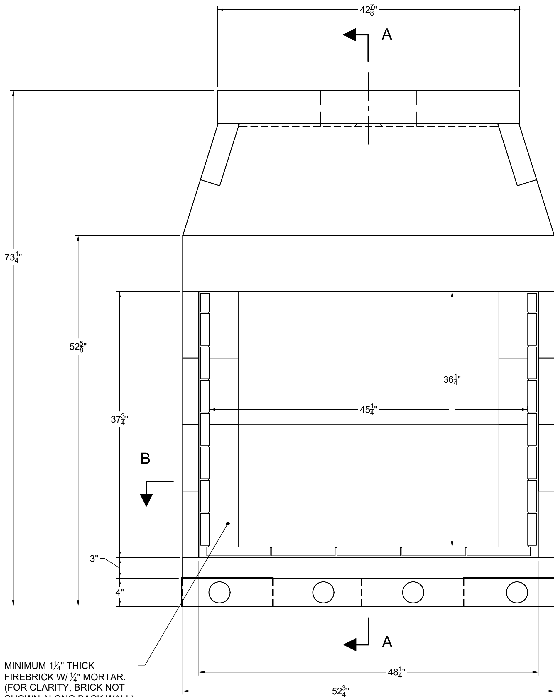
FRONT VIEW
