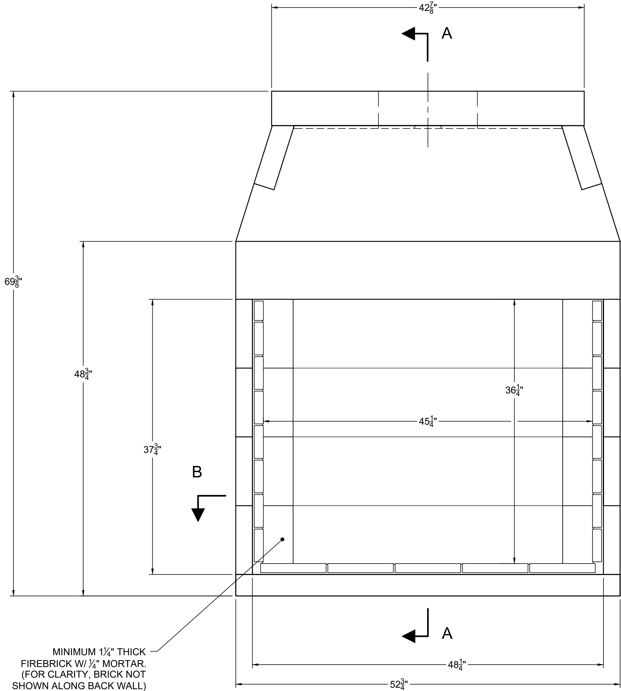
FRONT VIEW
