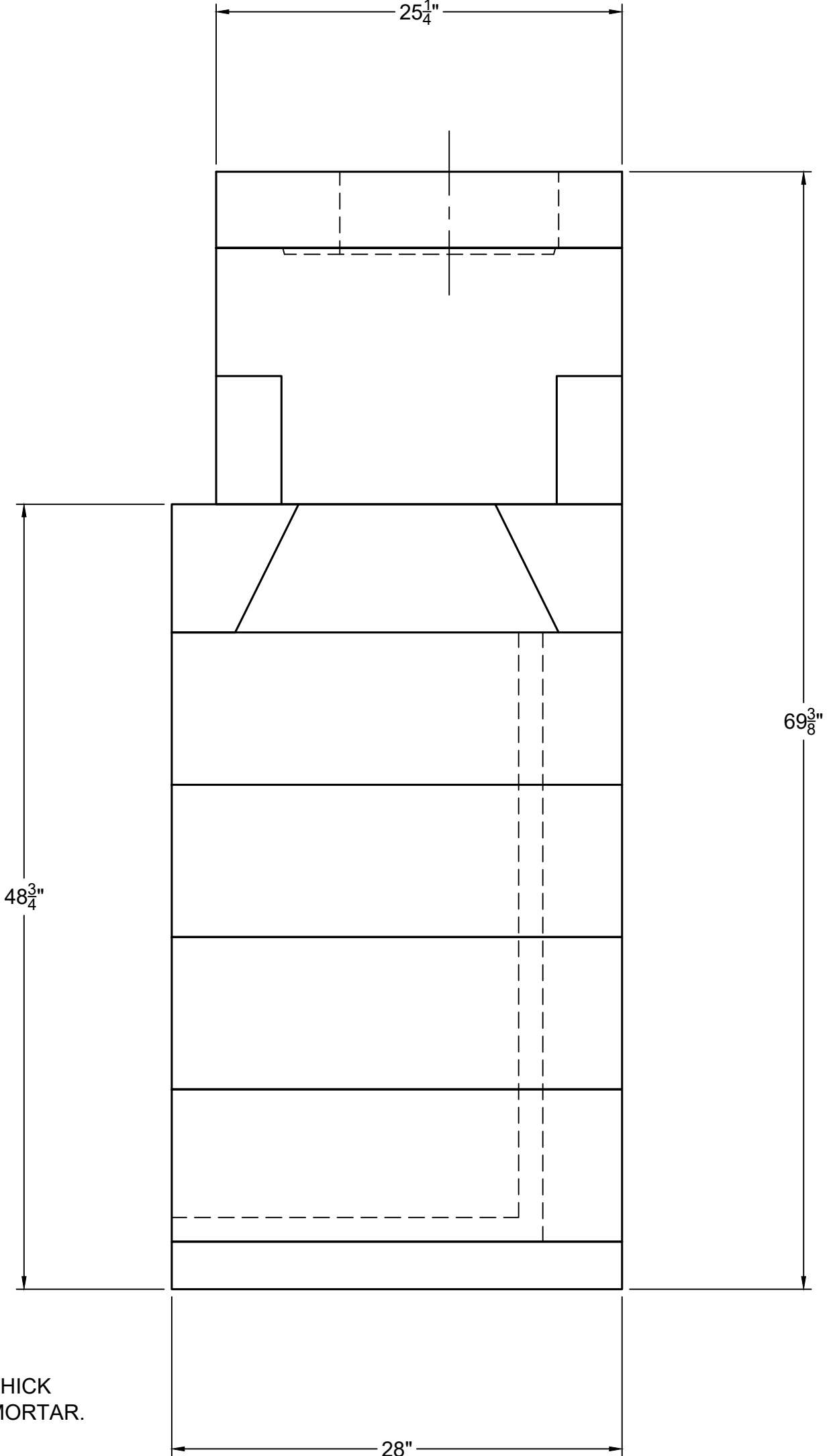
RIGHT-SIDE VIEW
