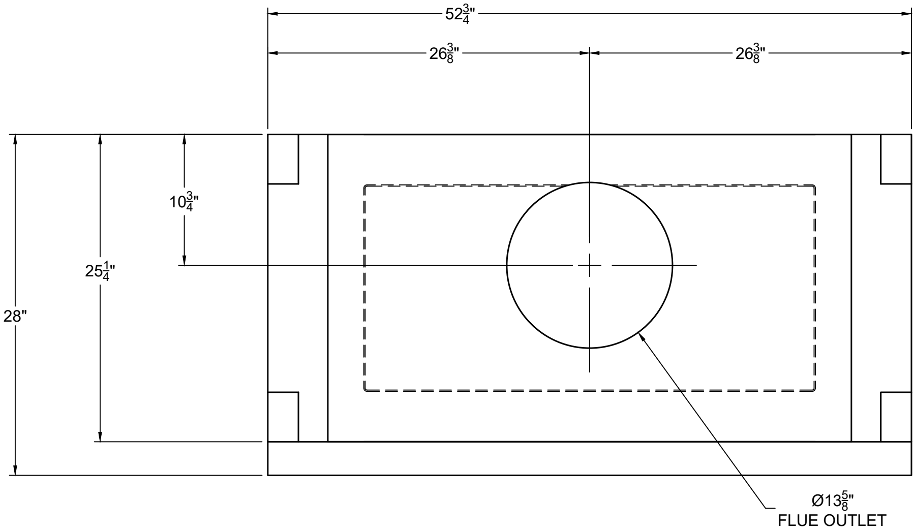
TOP VIEW
