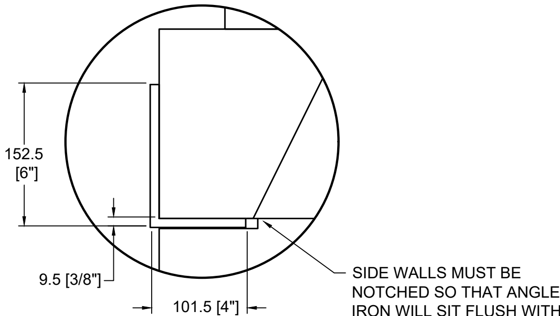
DETAIL A DAMPER SUPPORT ANGLE
