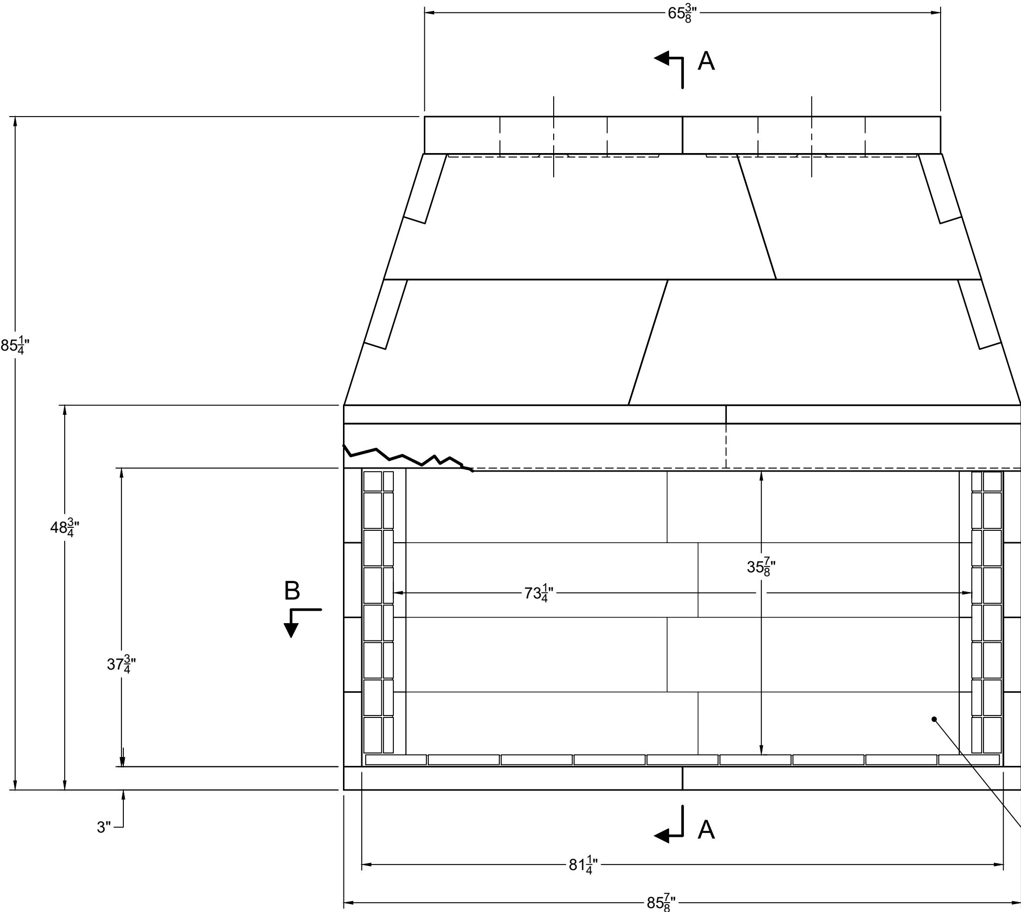
FRONT VIEW
