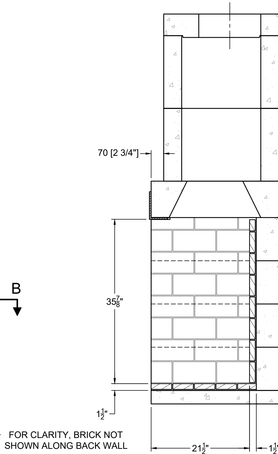
SECTION A-A VERTICAL FIREBRICK DETAIL
