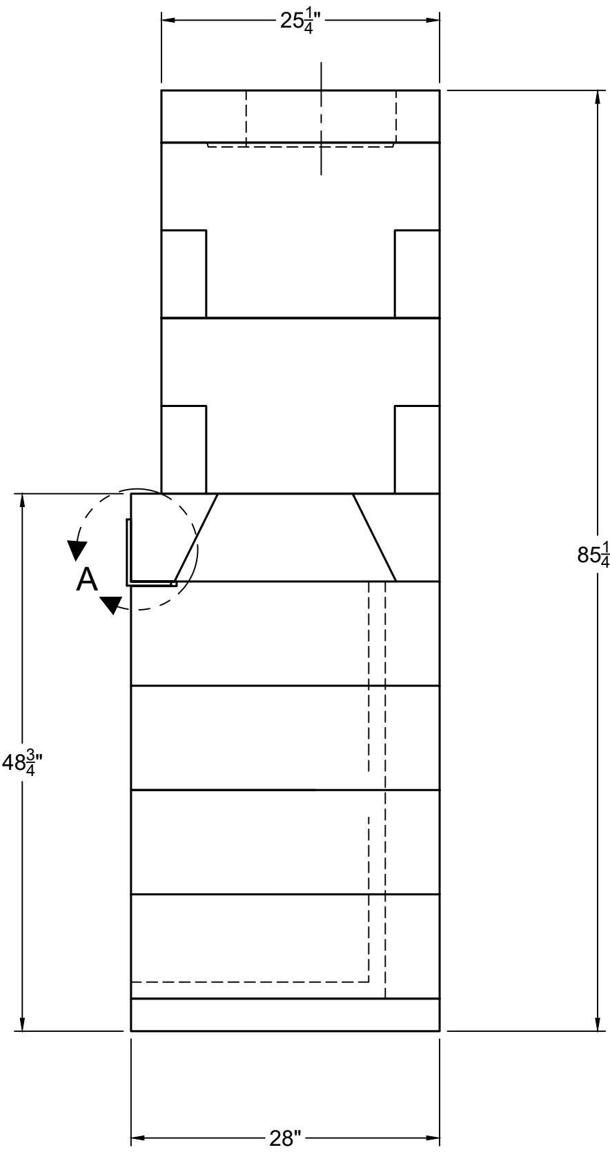
RIGHT-SIDE VIEW
