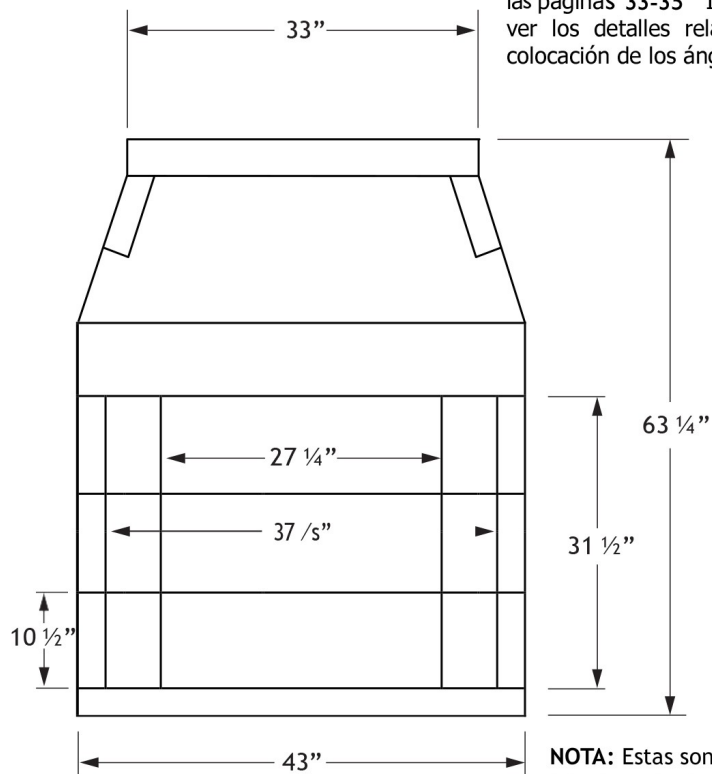
Vista frontal
