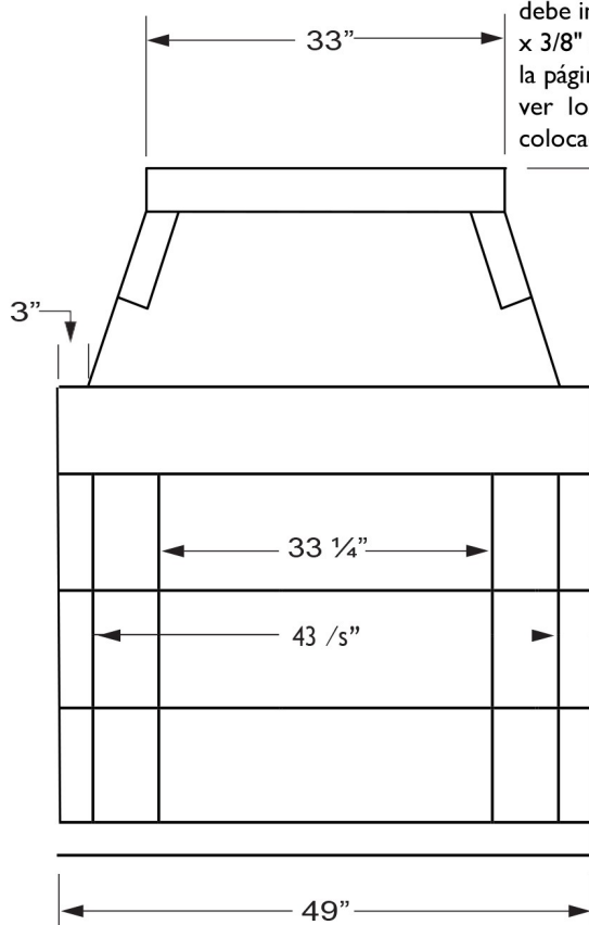
Vista frontal
