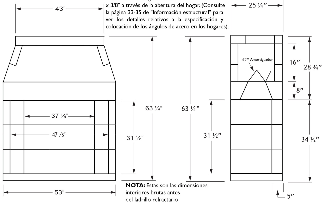
Vista frontal
