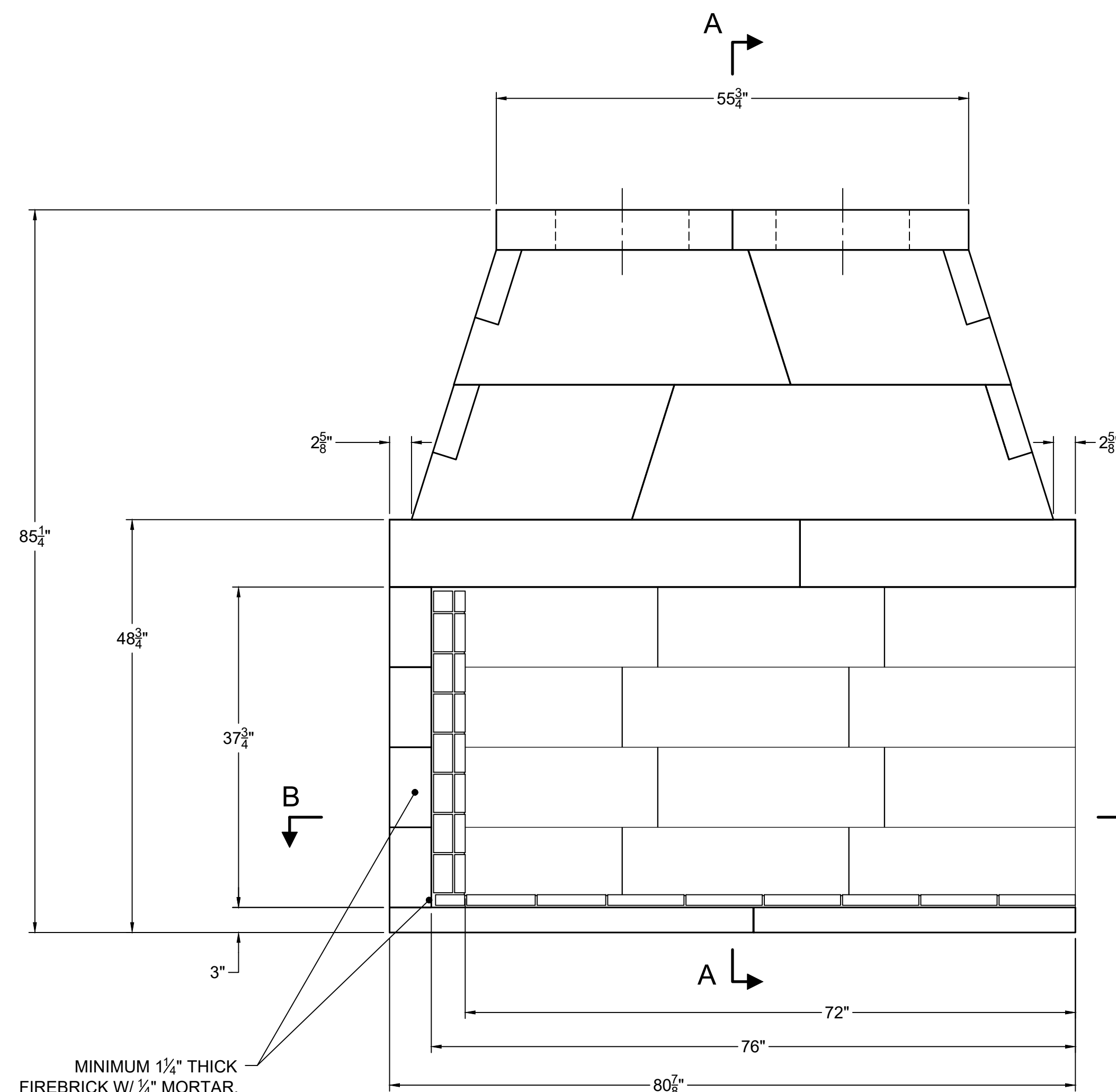
FRONT VIEW
