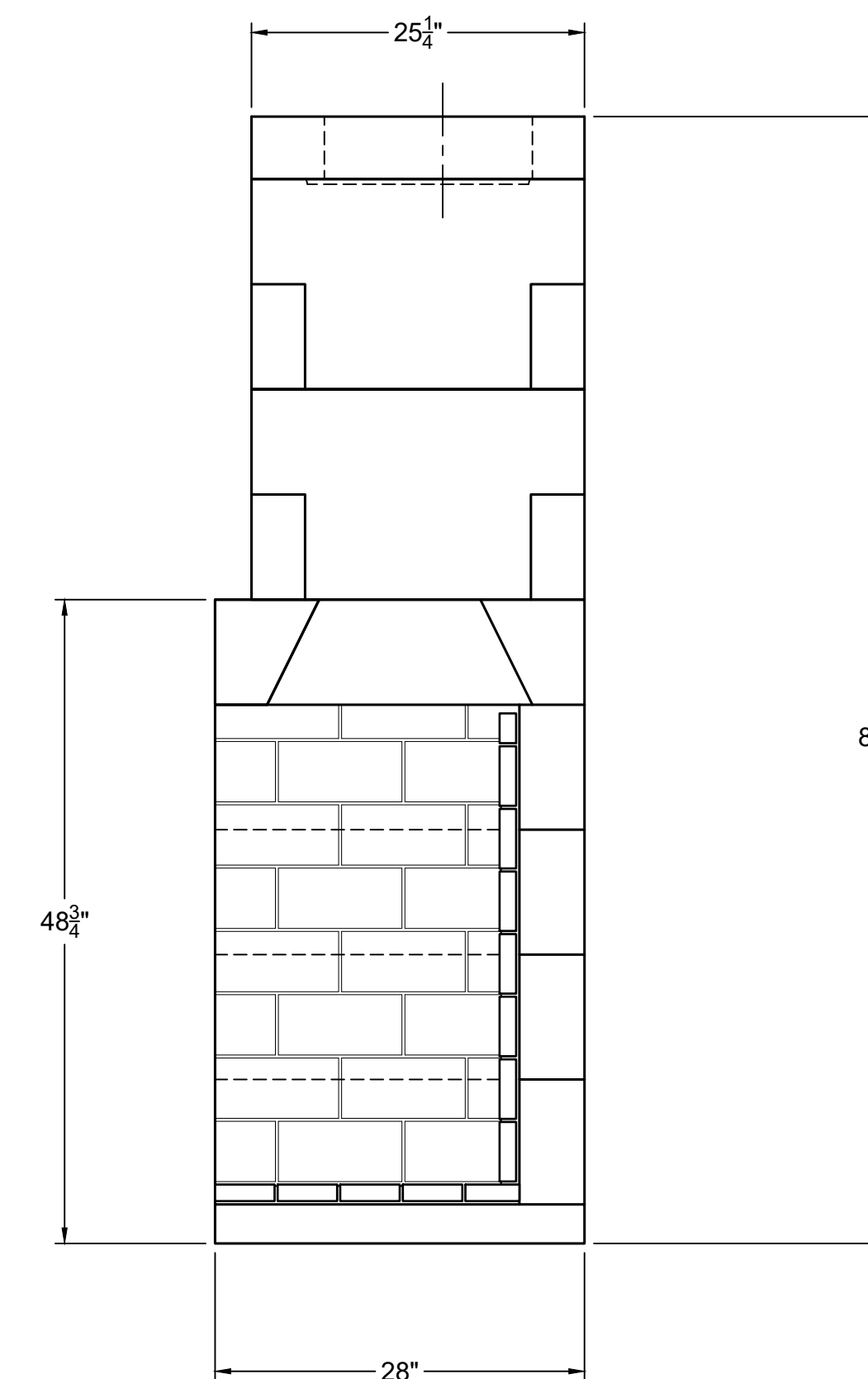
RIGHT-SIDE VIEW
