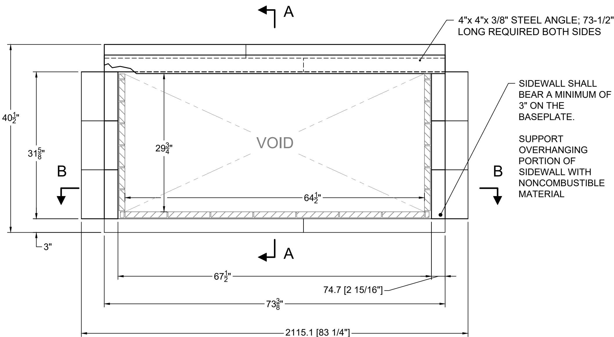
FRONT VIEW
