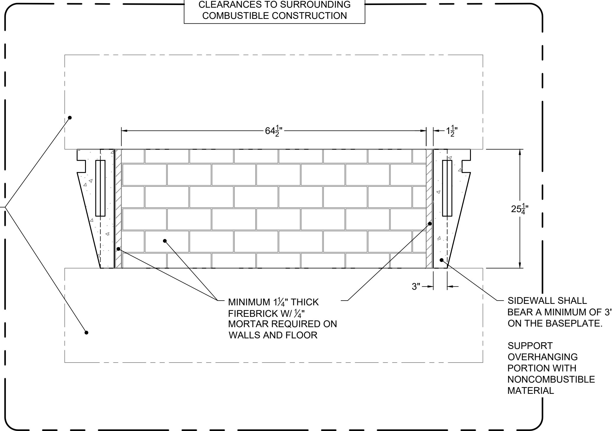
SECTION B-B
