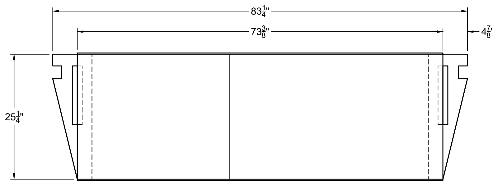
TOP VIEW
