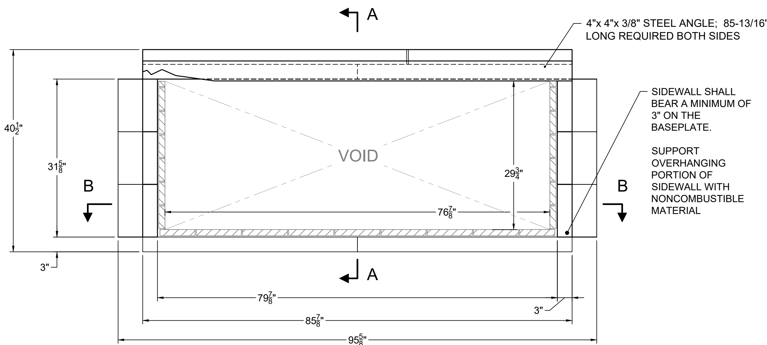
FRONT VIEW
