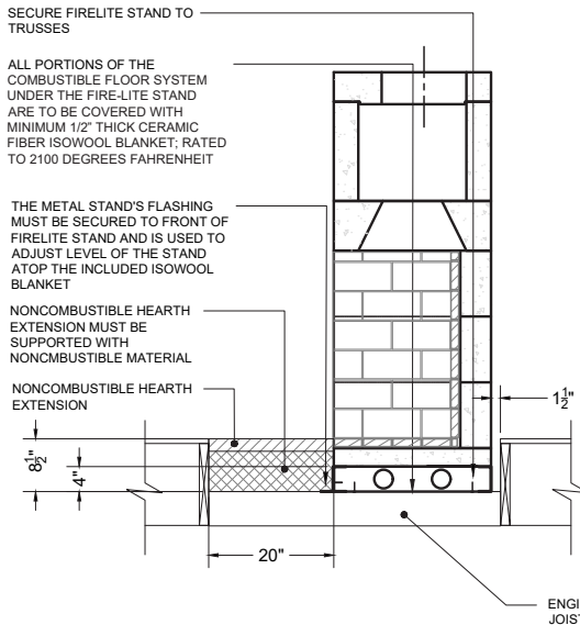
STANDARD & MAGNUM RECESSED FIRELITE APPLICATION
