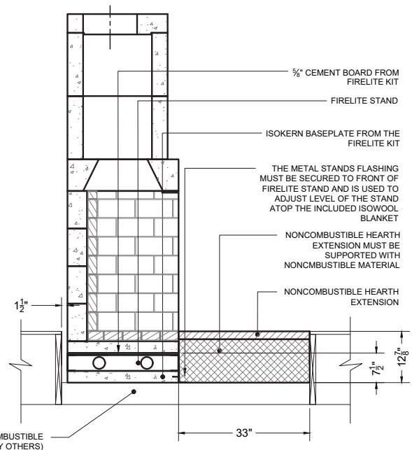
MAGNUM 60/72 RECESSED FIRELITE APPLICATION
