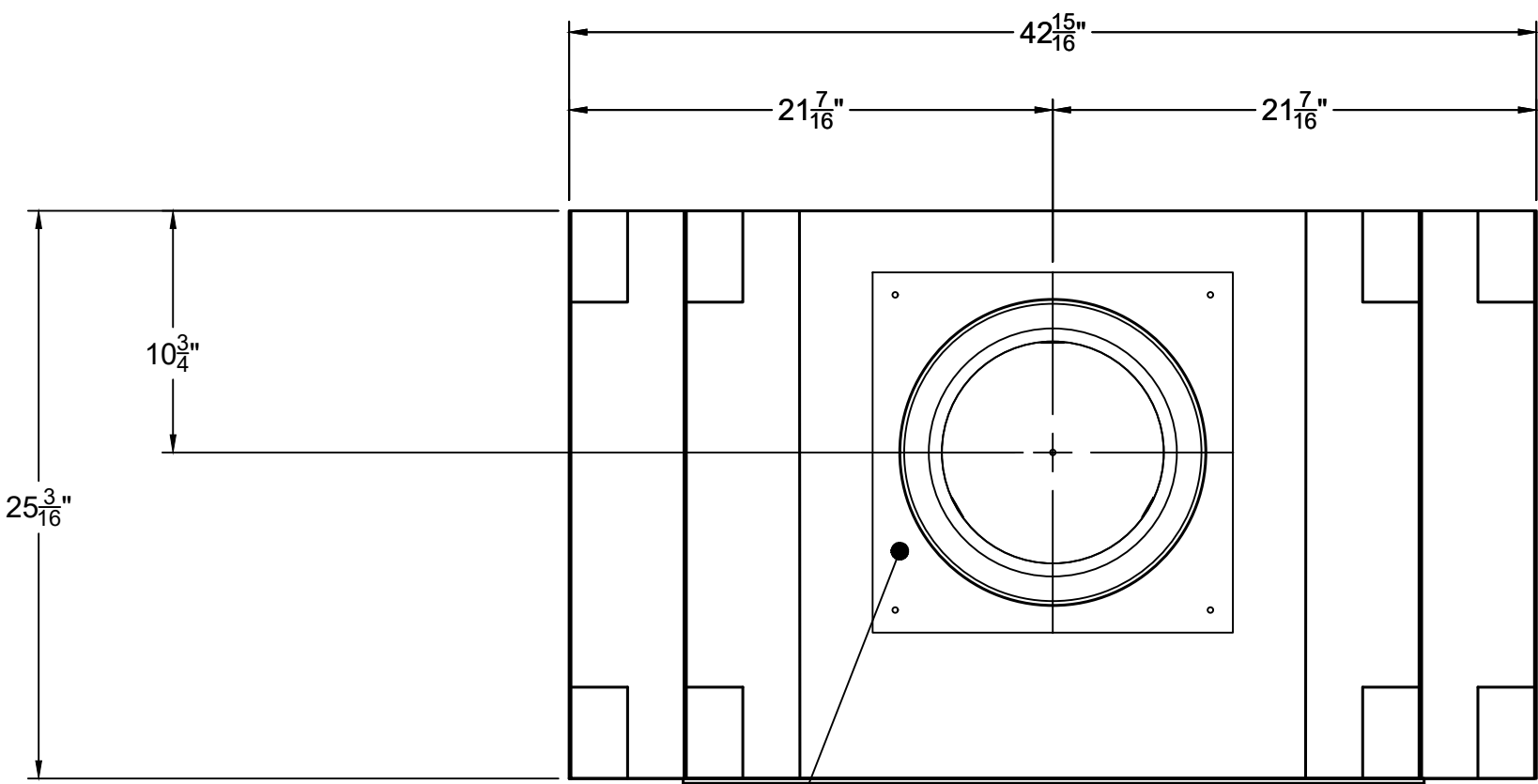
TOP VIEW
