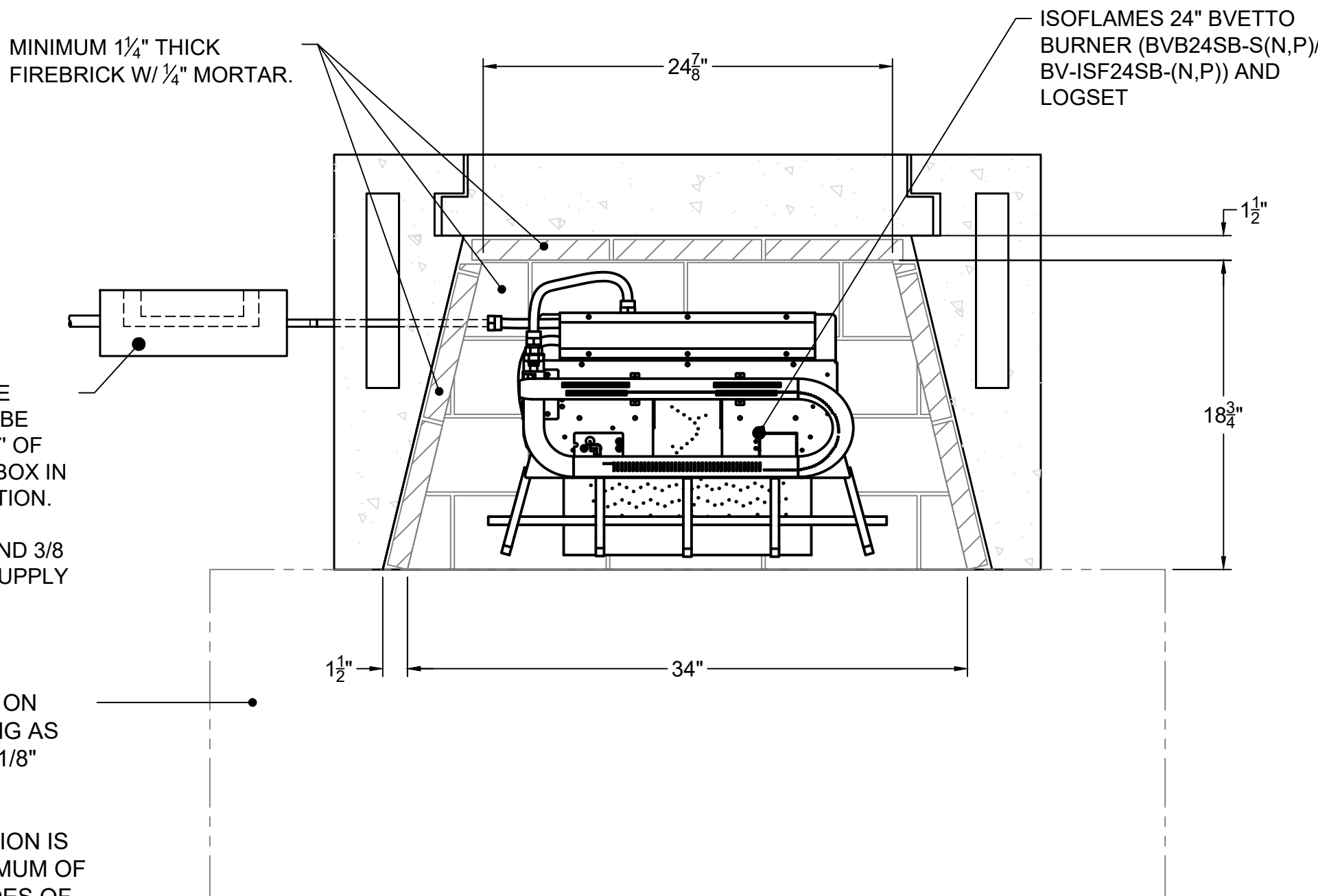
SECTION B-B
