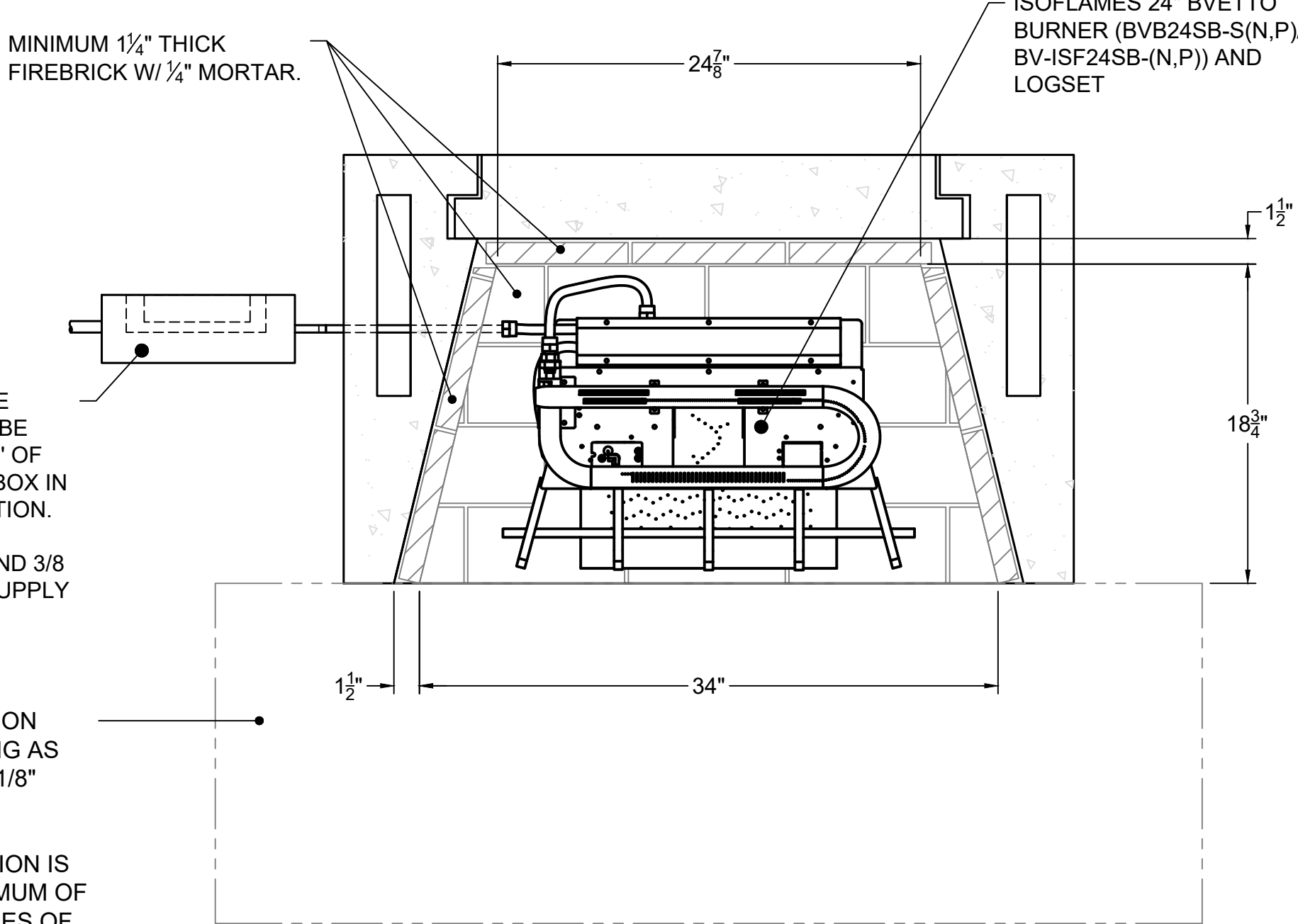
SECTION B-B
