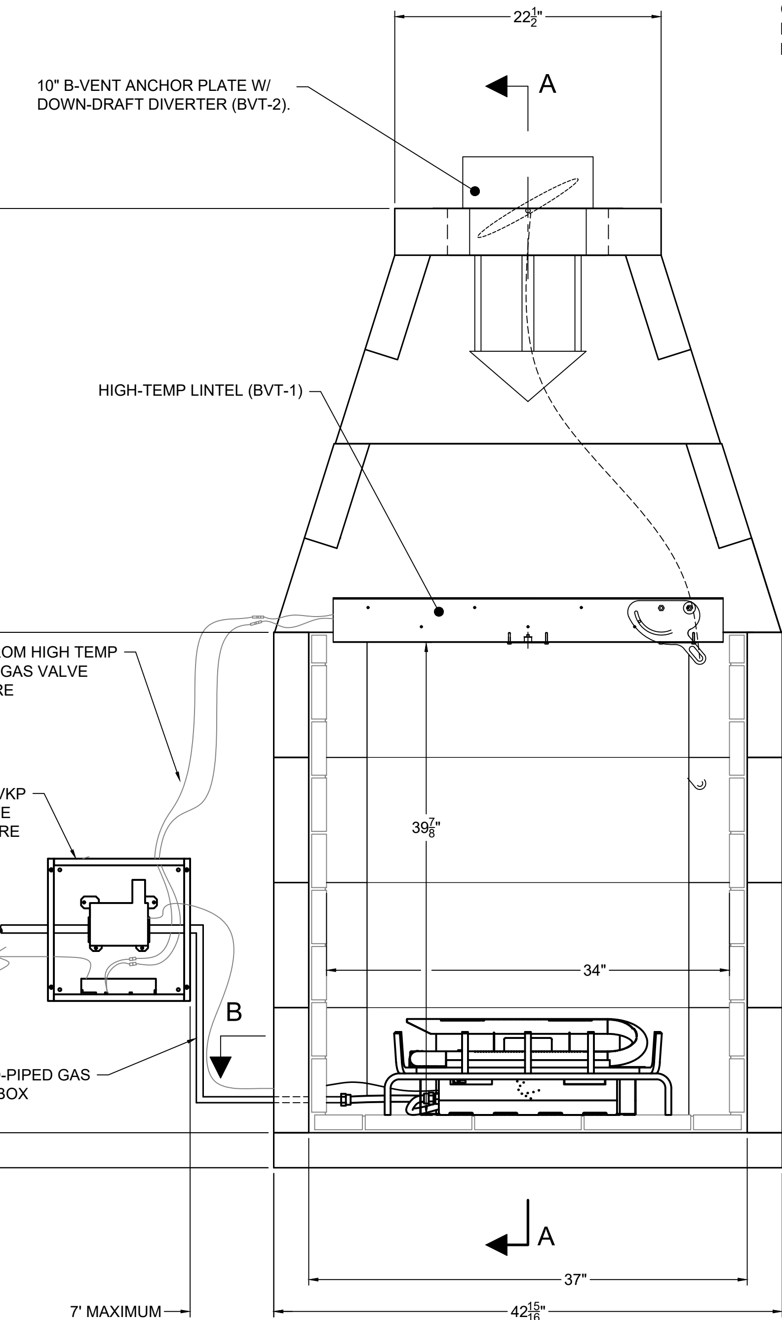
FRONT VIEW
