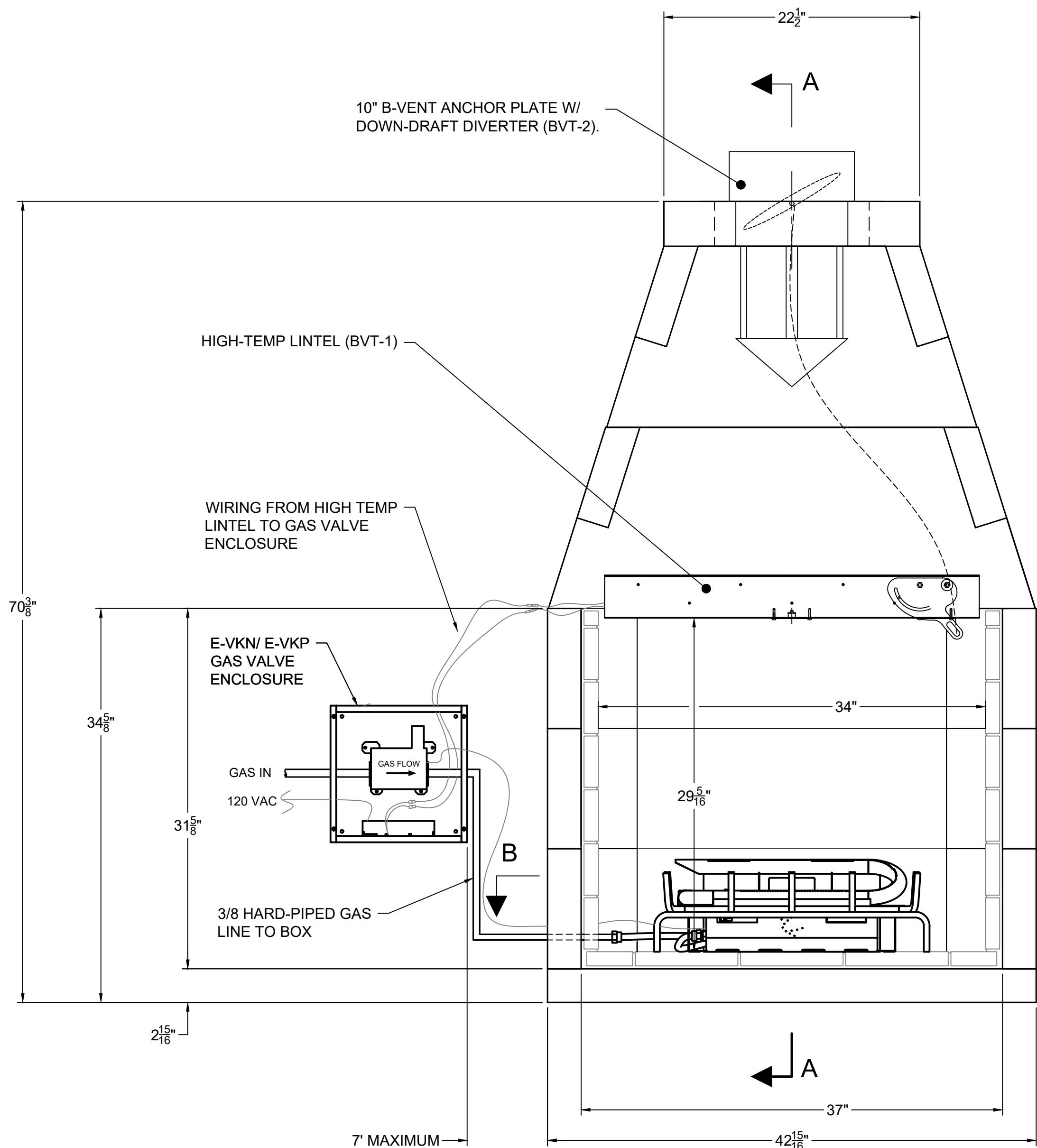
FRONT VIEW BRICK NOT SHOWN ON REAR WALL IN THIS VIEW
