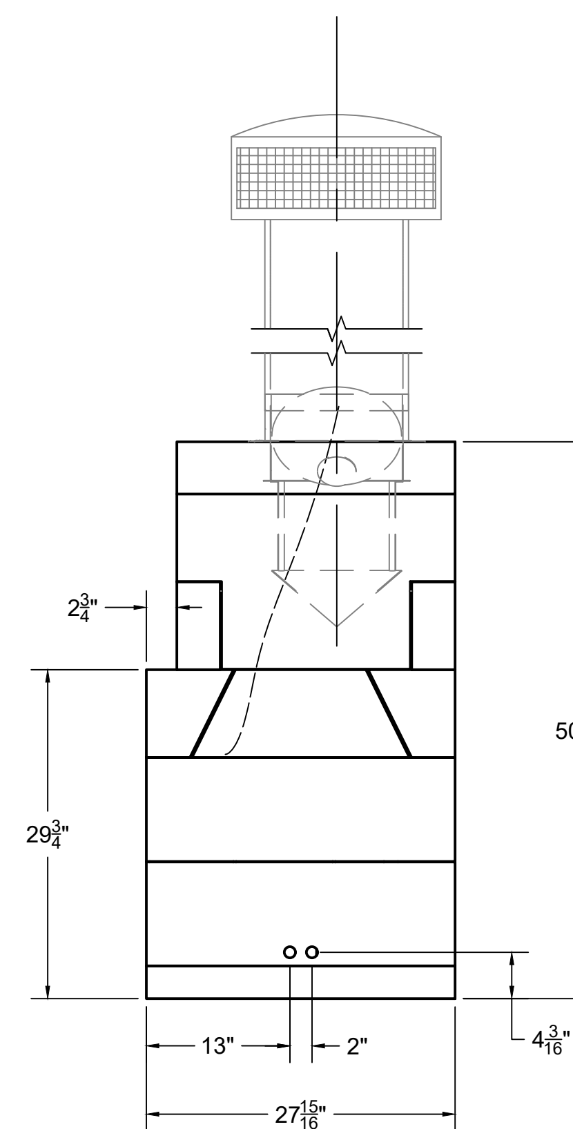
RIGHT
