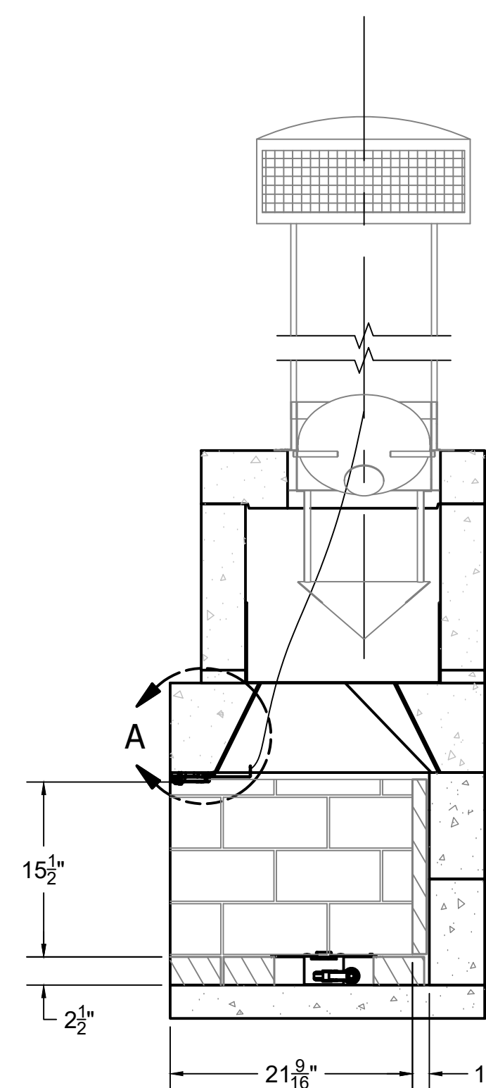
SECTION B-B
