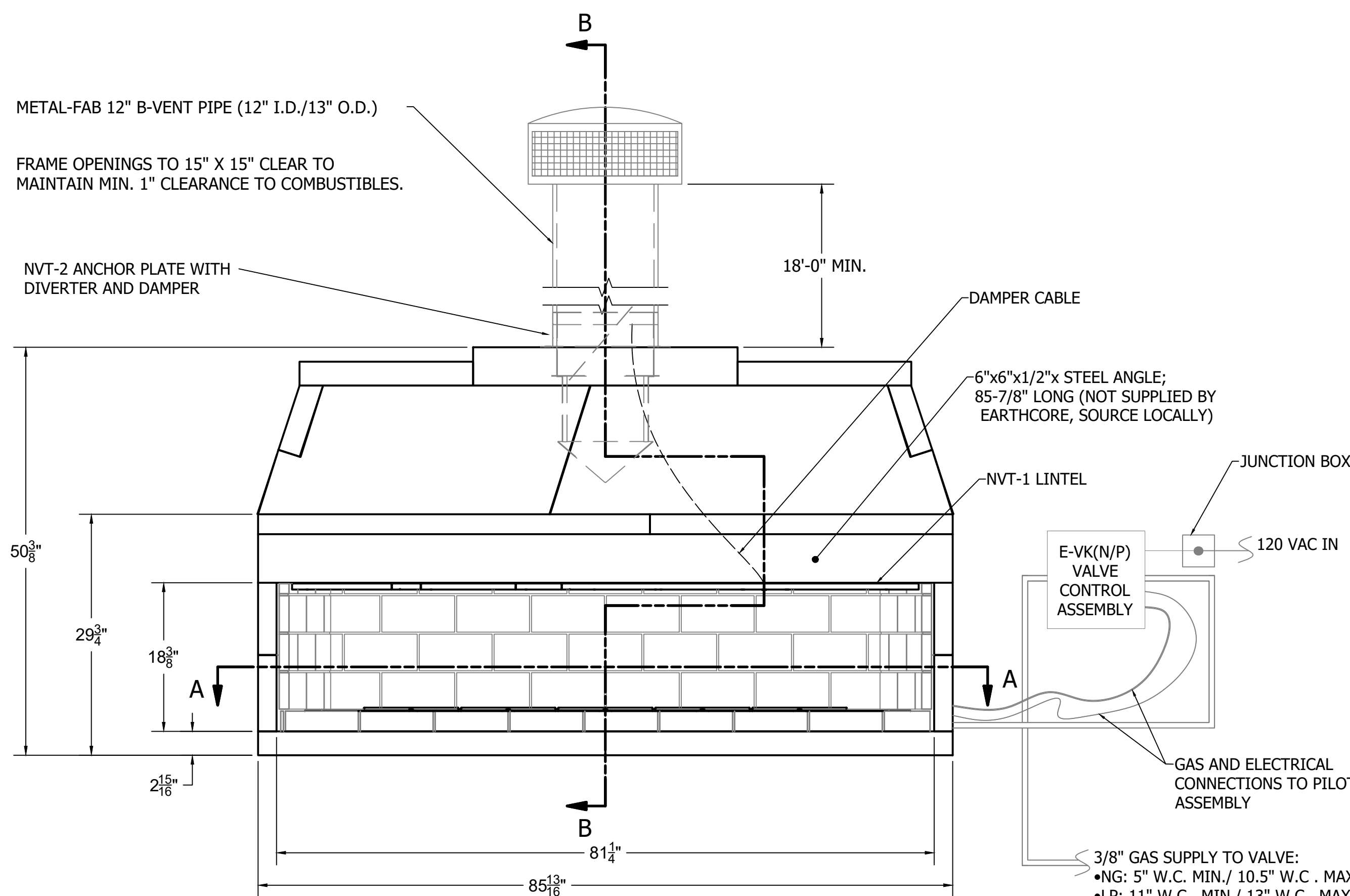
FRONT
