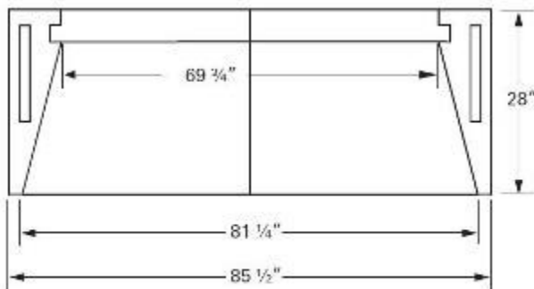
Plan View
