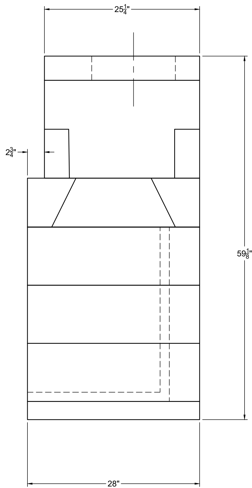
RIGHT SIDE VIEW
