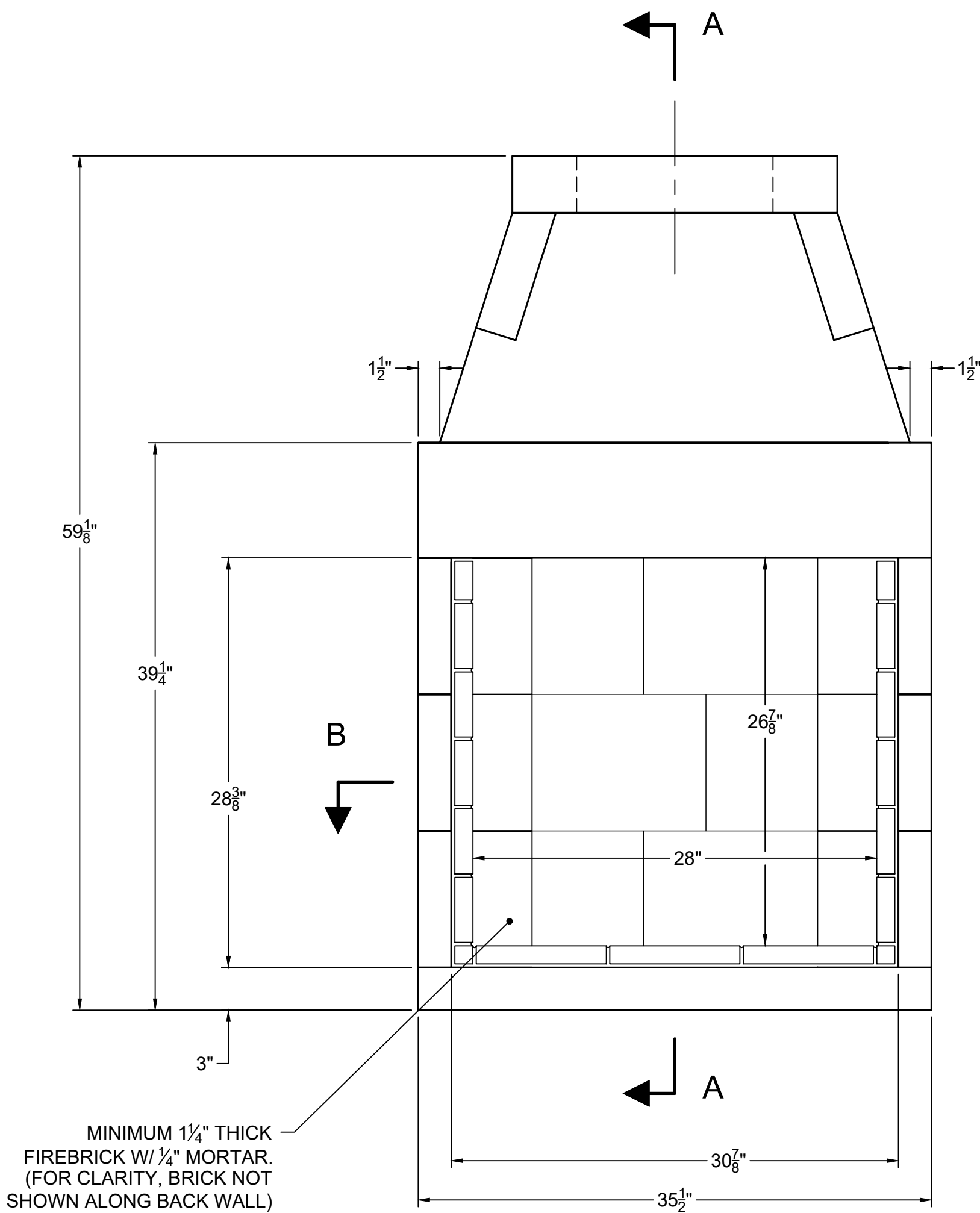
FRONT VIEW
