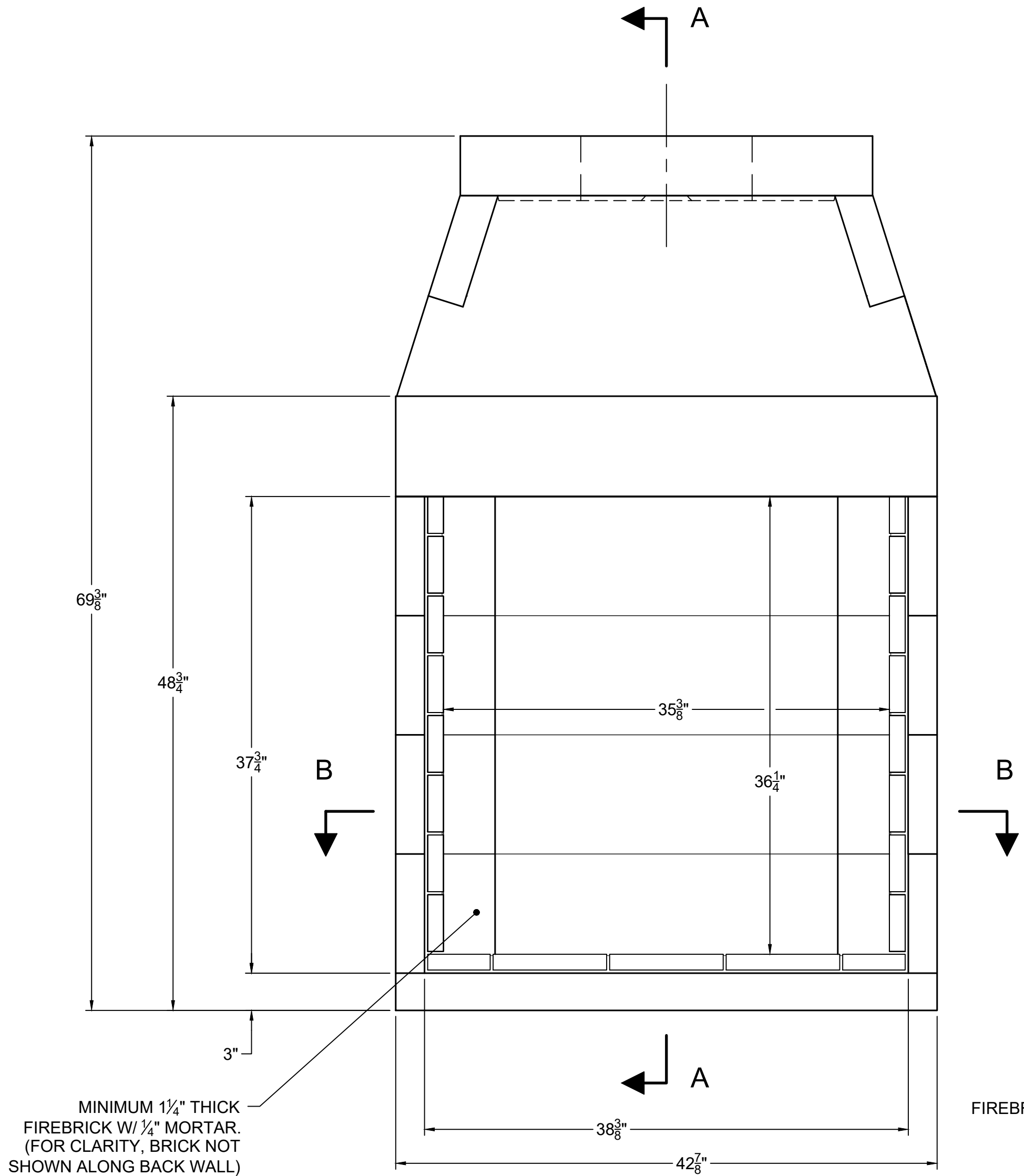
FRONT VIEW
