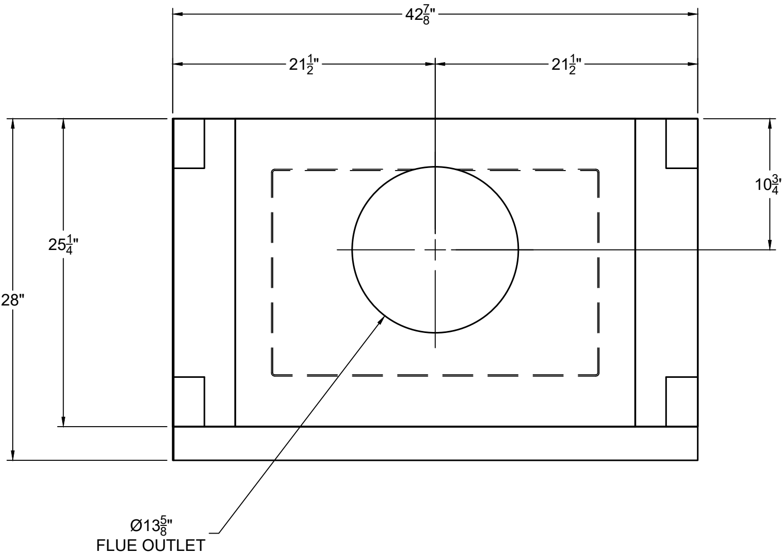
TOP VIEW
