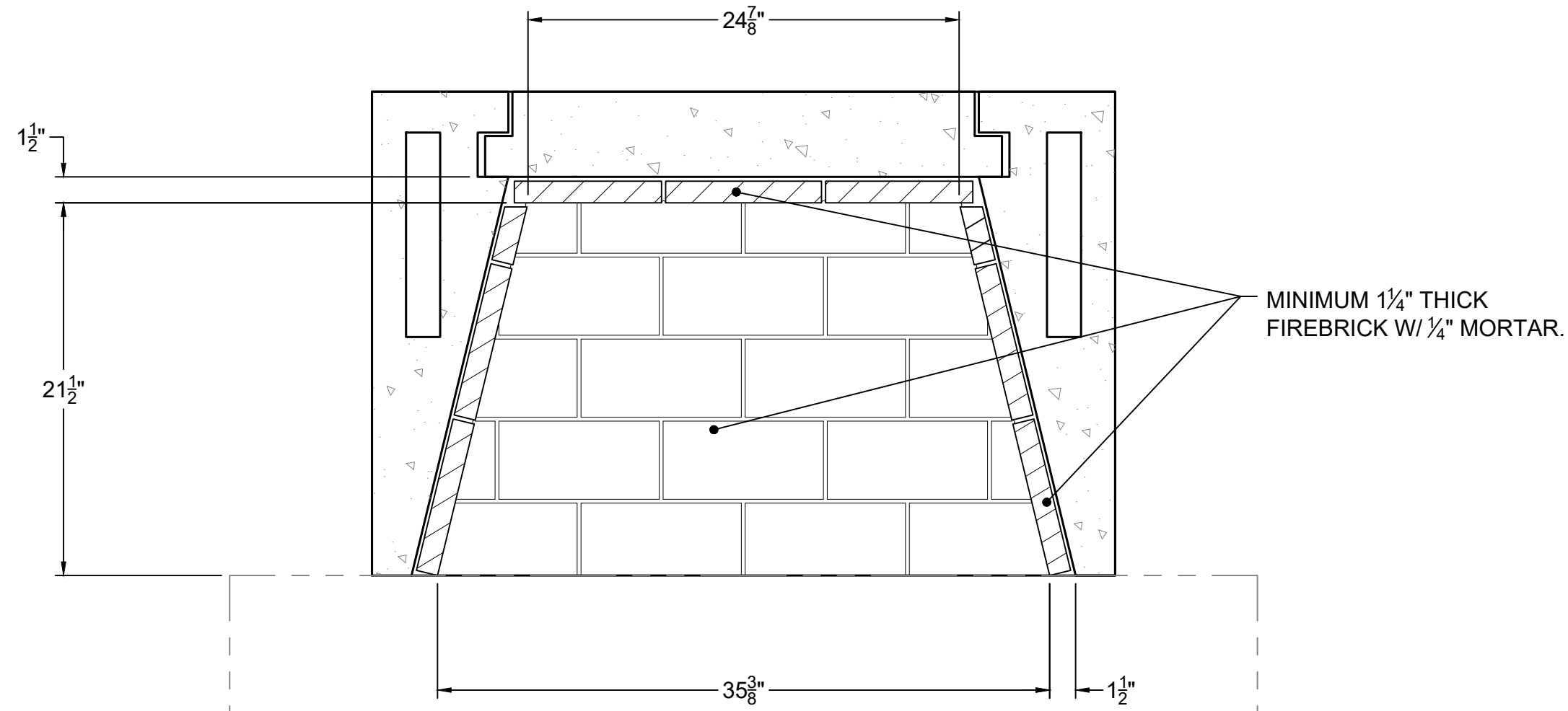
SECTION B-B HORIZONTAL FIREBRICK DETAIL
