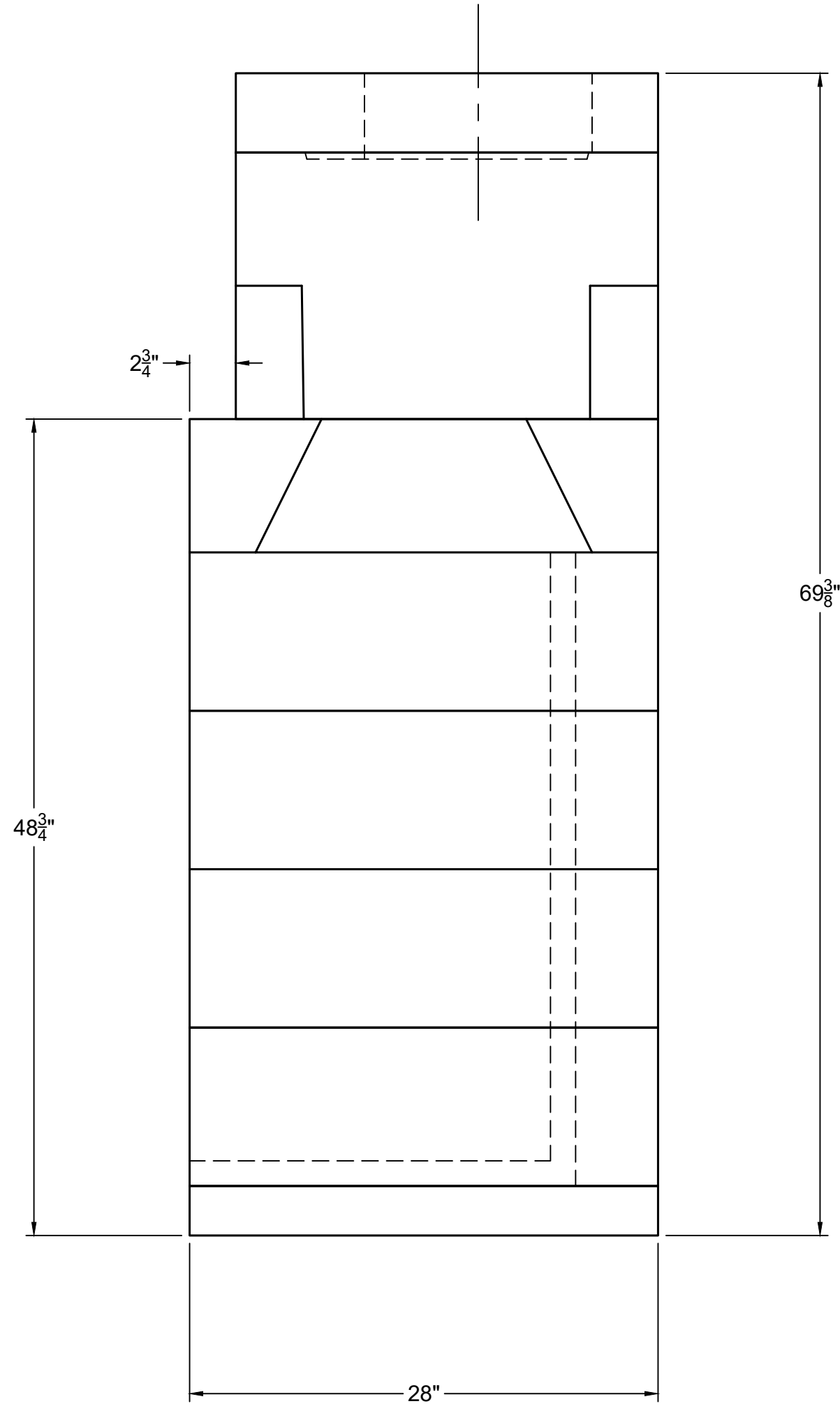
RIGHT-SIDE VIEW
