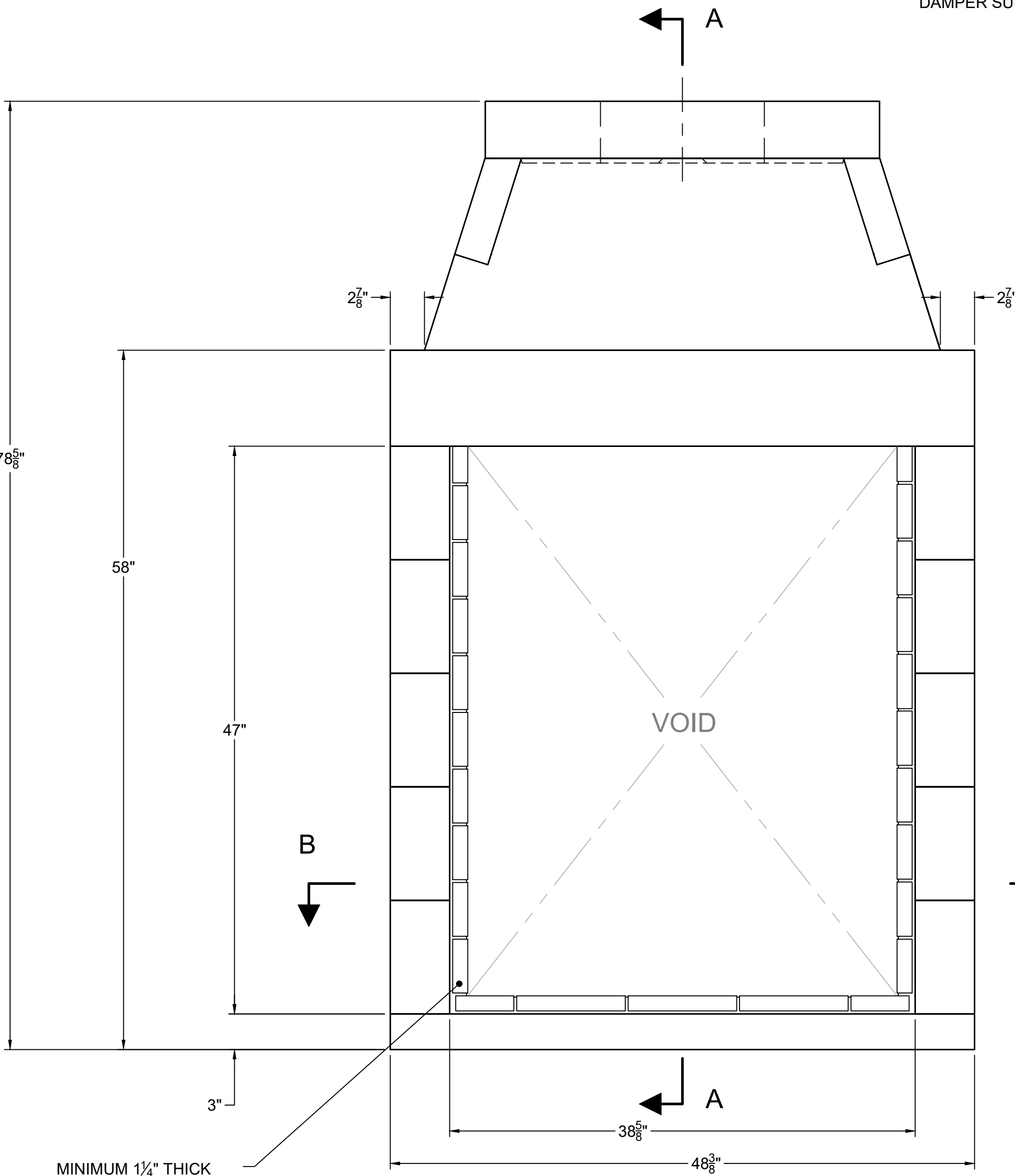
FRONT VIEW
