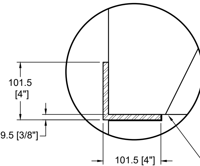
DETAIL A DAMPER SUPPORT ANGLE
