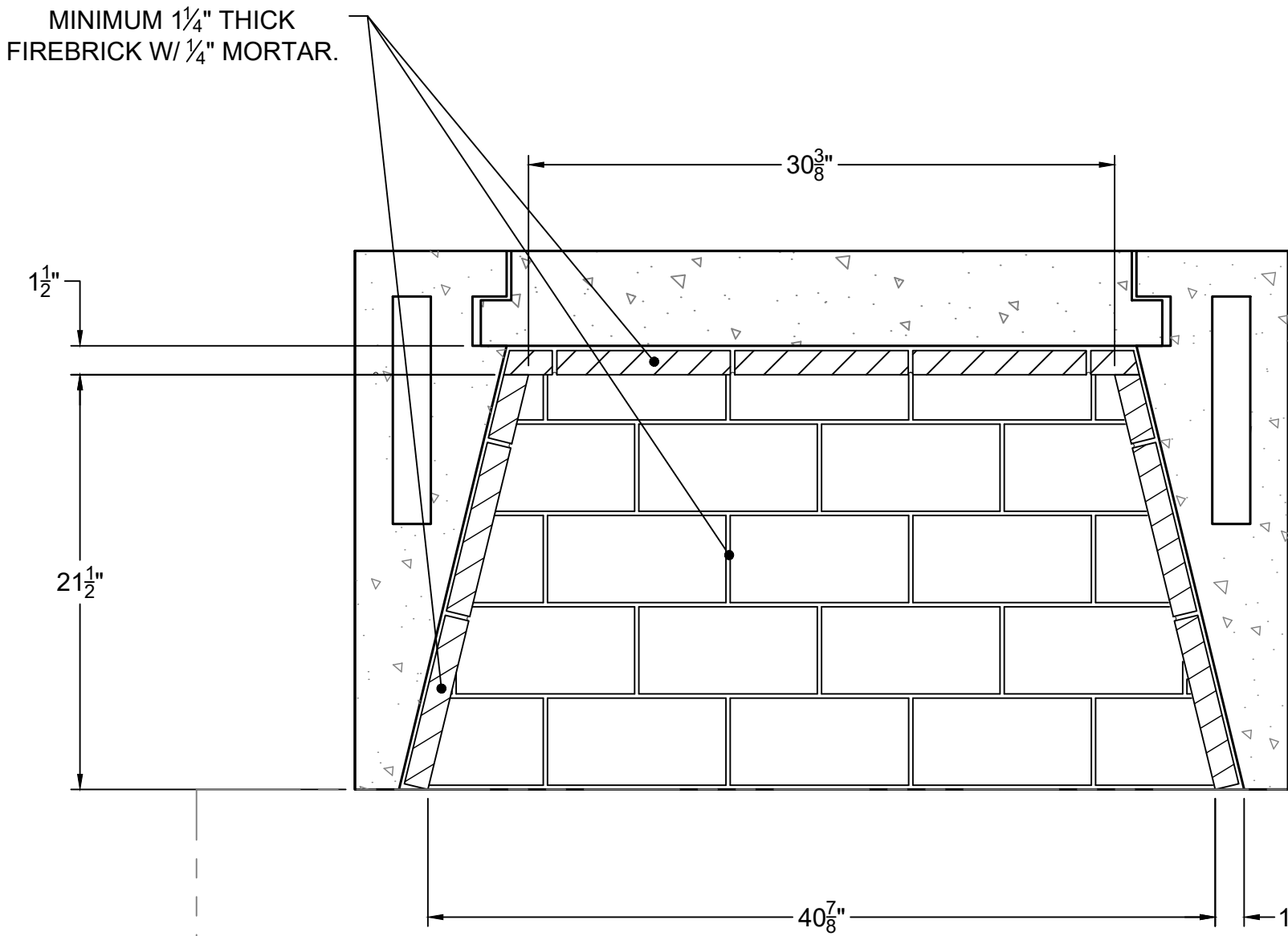
SECTION B-B HORIZONTAL FIREBRICK DETAIL
