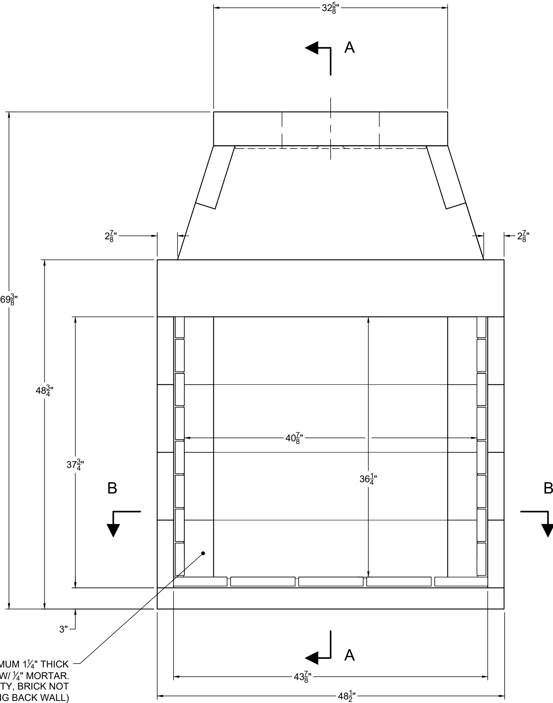
FRONT VIEW
