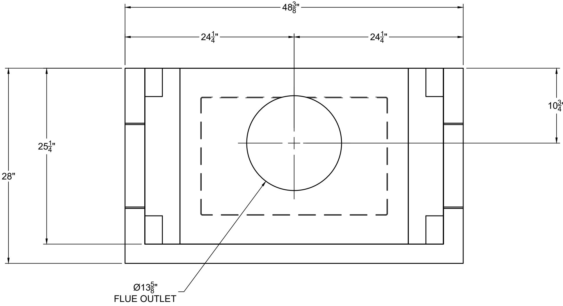
TOP VIEW
