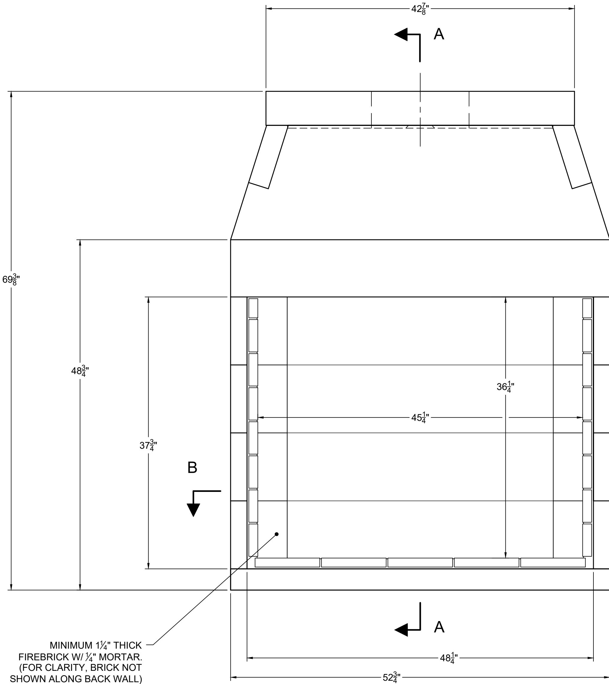
FRONT VIEW
