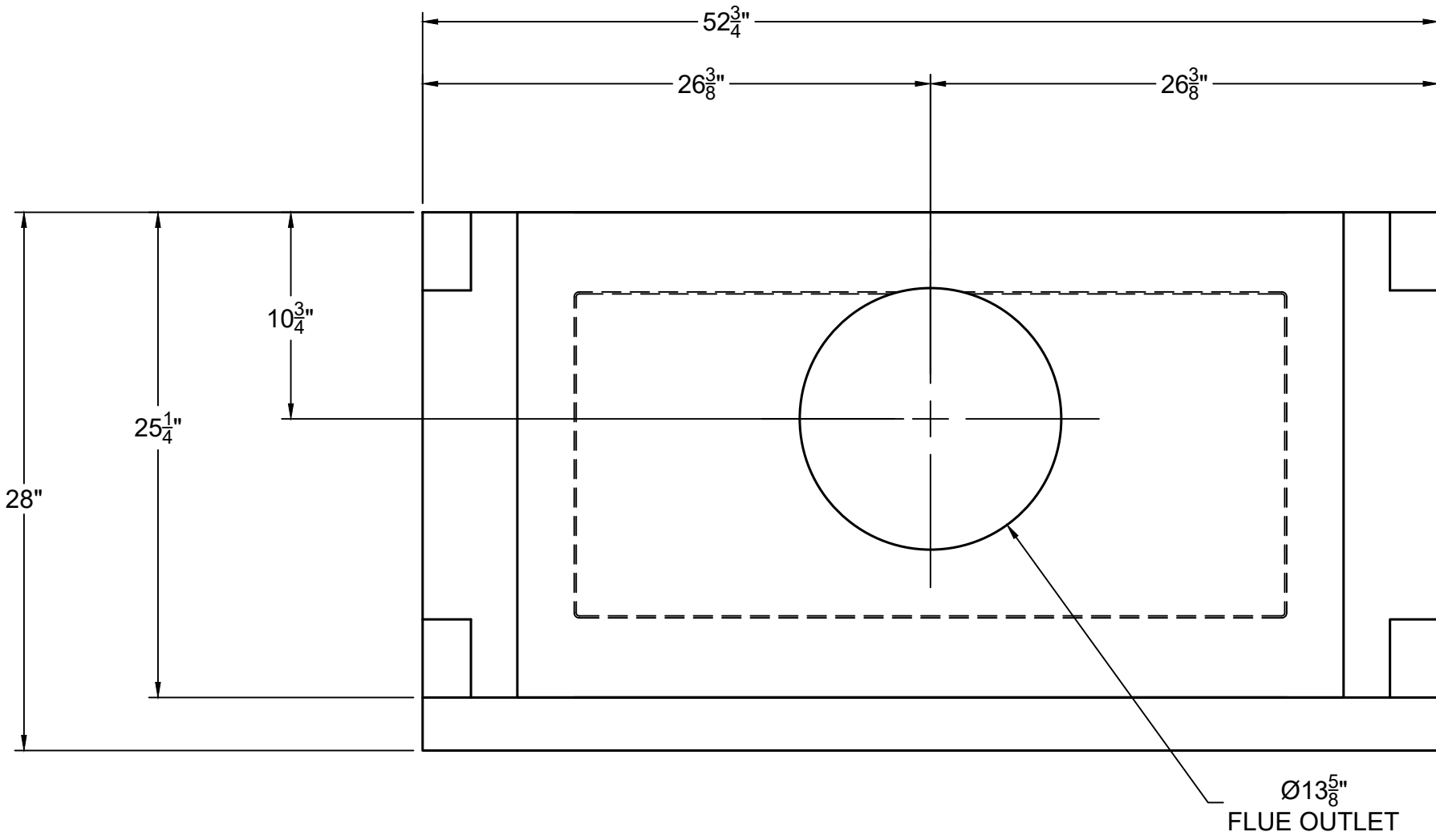
TOP VIEW
