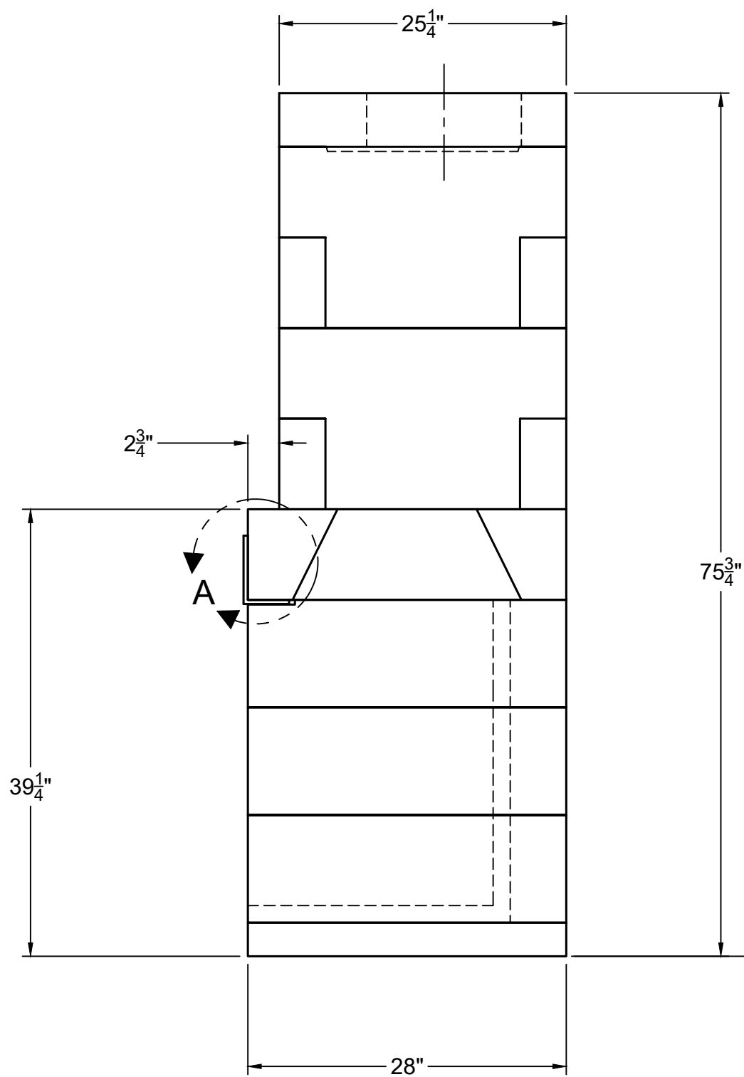
RIGHT-SIDE VIEW
