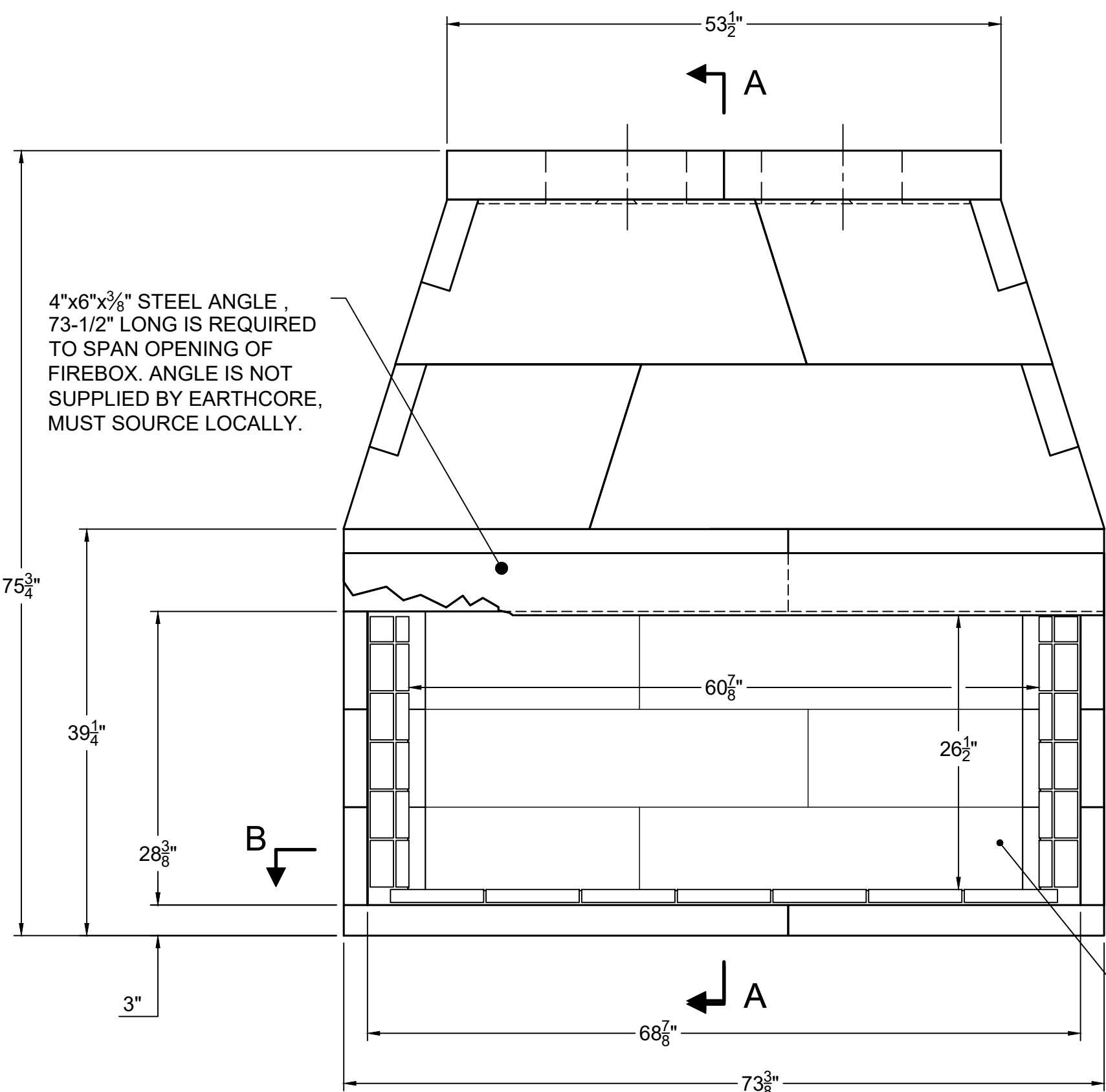
FRONT VIEW
