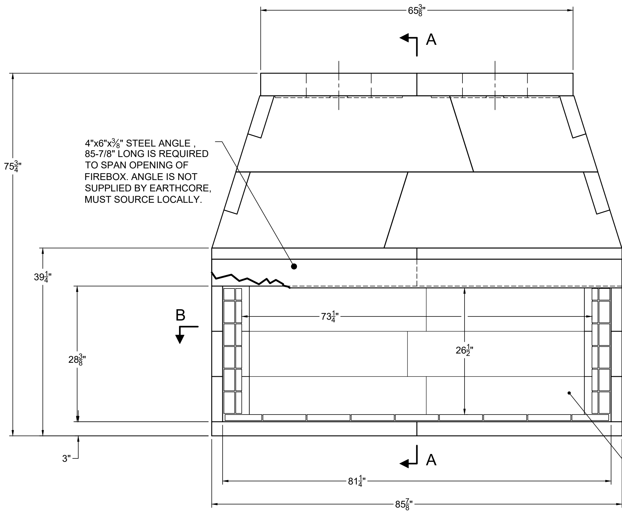
FRONT VIEW
