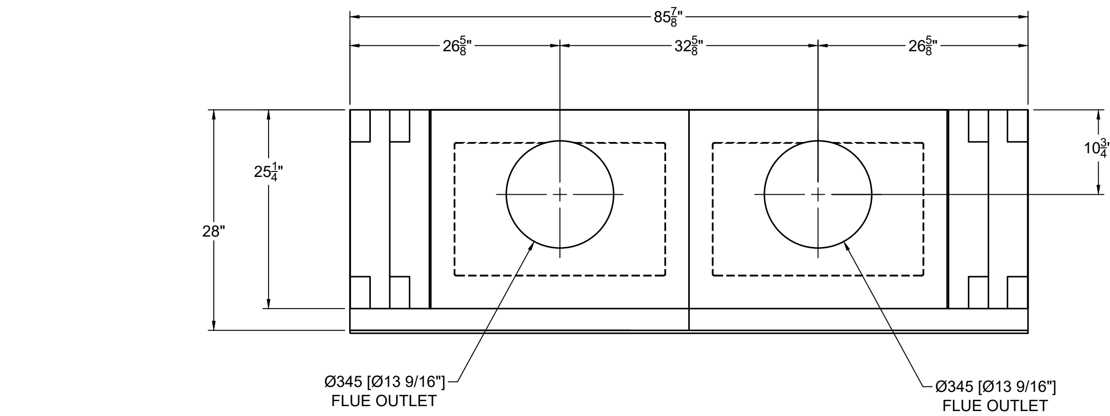
TOP VIEW
