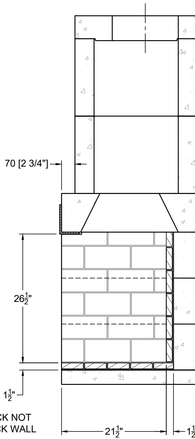
SECTION A-A VERTICAL FIREBRICK DETAIL
