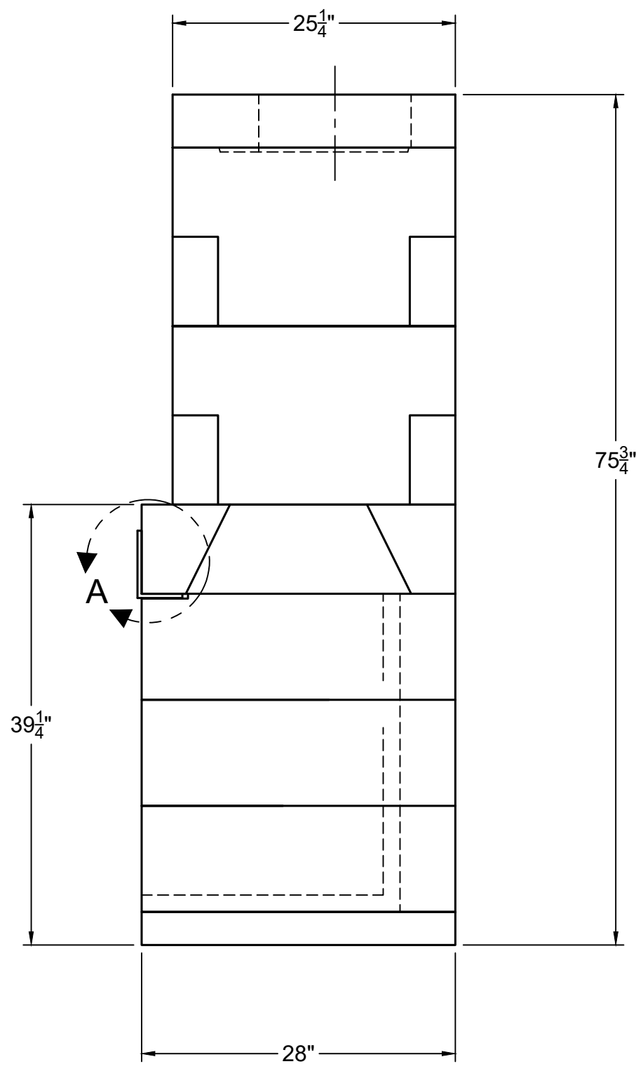
RIGHT-SIDE VIEW
