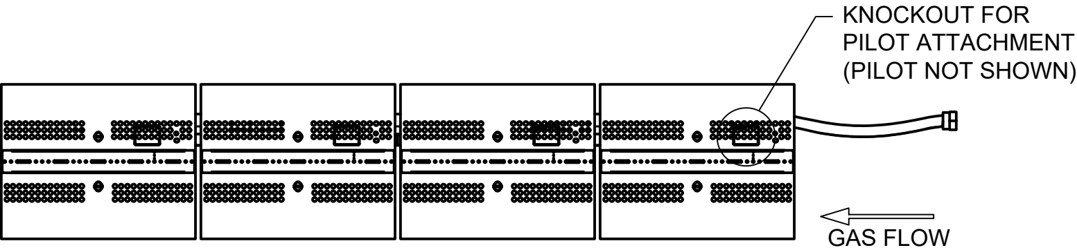
TOP VIEW
