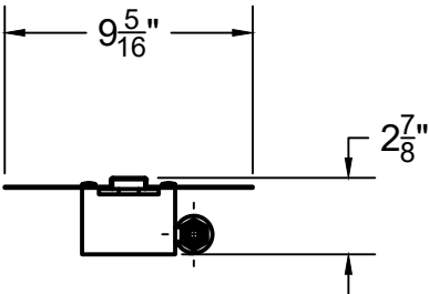
RIGHT-SIDE VIEW
