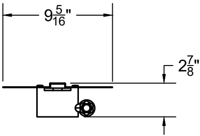
RIGHT-SIDE VIEW
