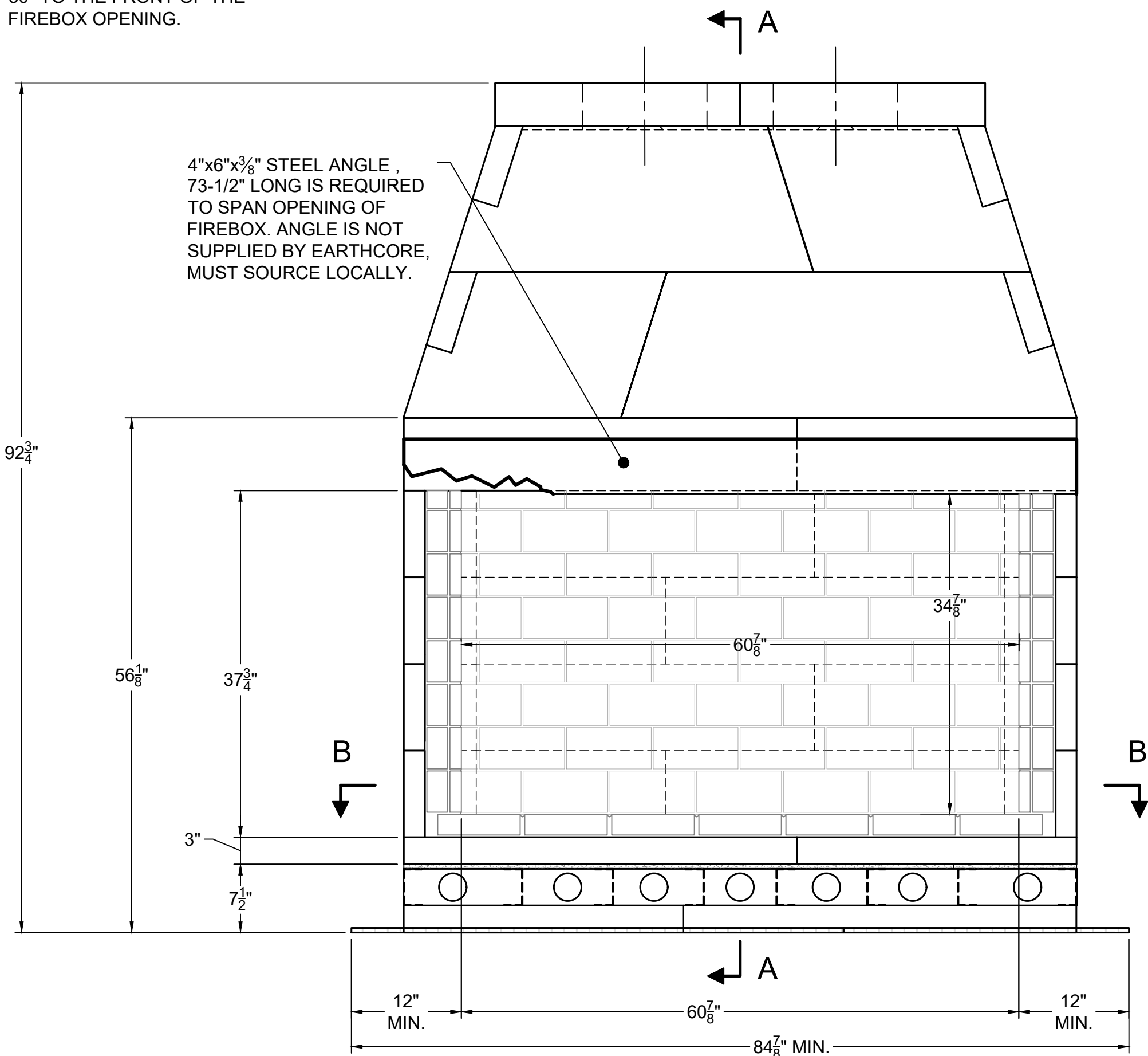
FRONT VIEW *MS-M-60 FLASHING NOT SHOWN IN VIEW
