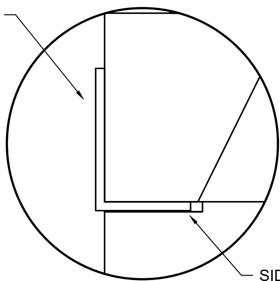
DETAIL A DAMPER SUPPORT ANGLE SCALE: 3"=1'-0"
