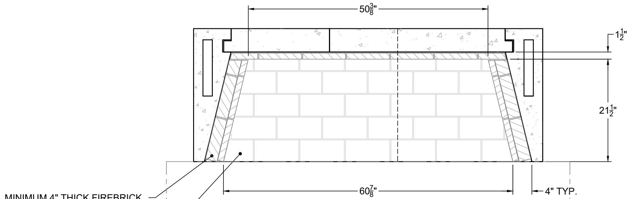
SECTION B-B
