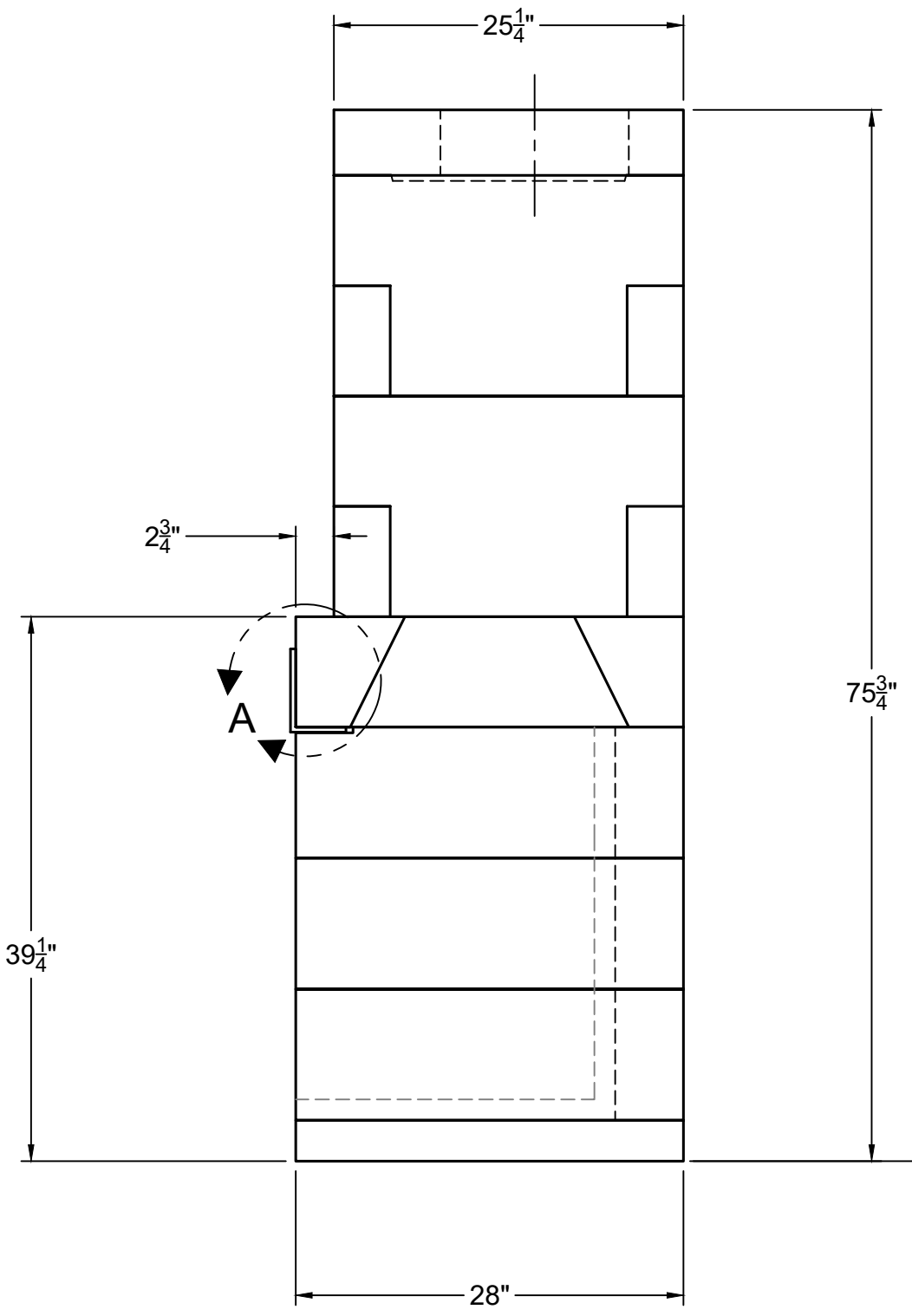
RIGHT-SIDE VIEW
