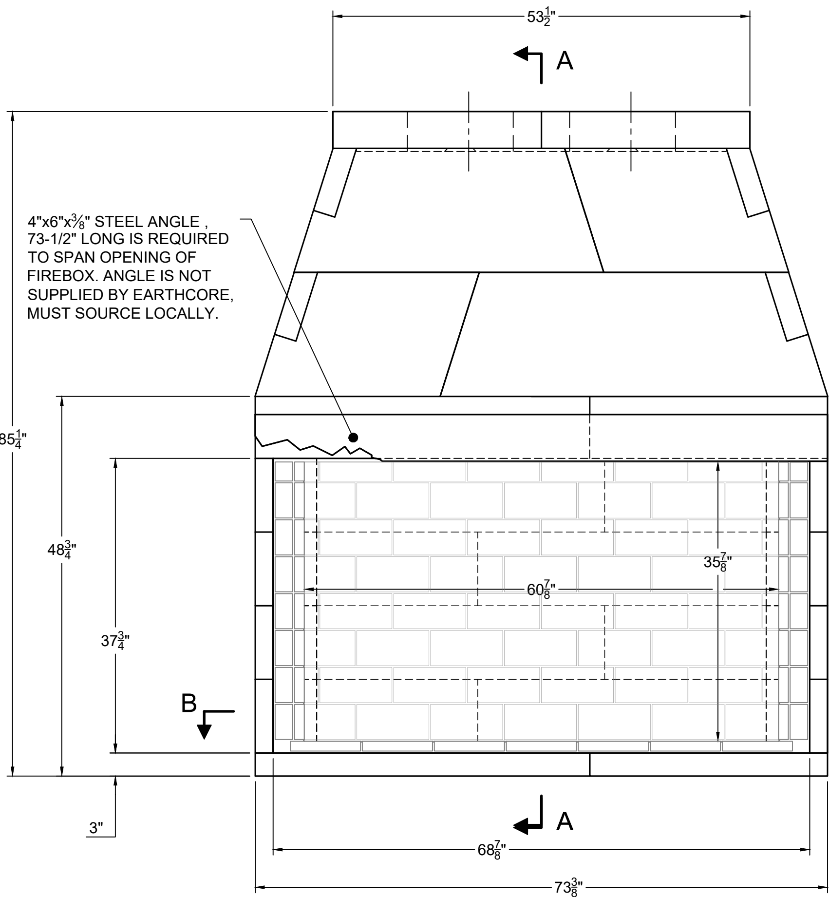
FRONT VIEW
