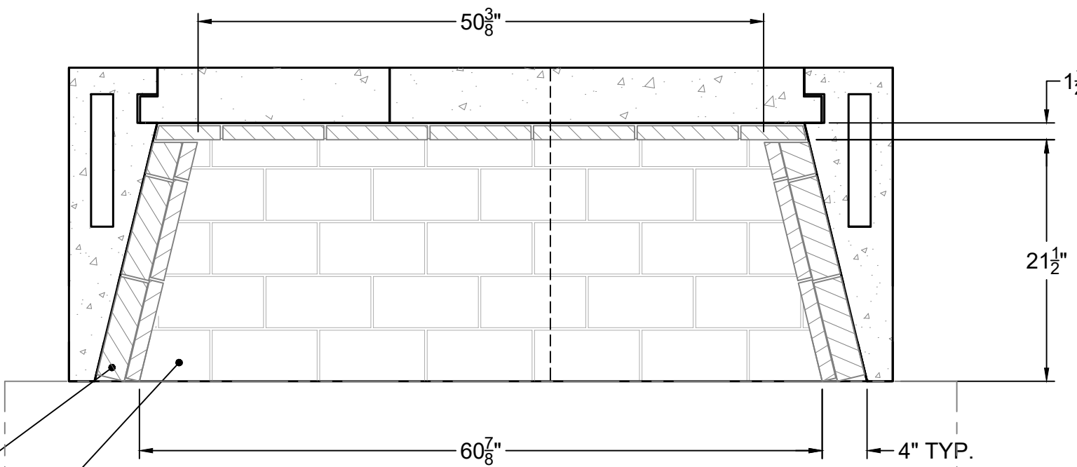
SECTION B-B HORIZONTAL FIREBRICK DETAIL
