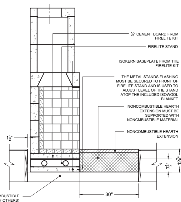
MAGNUM 60/72 RECESSED FIRELITE + APPLICATION
