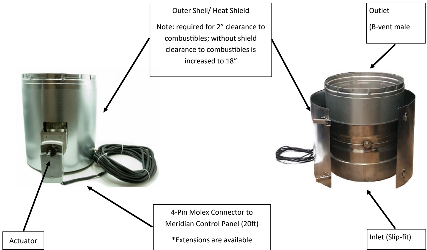
Damper Assembly
