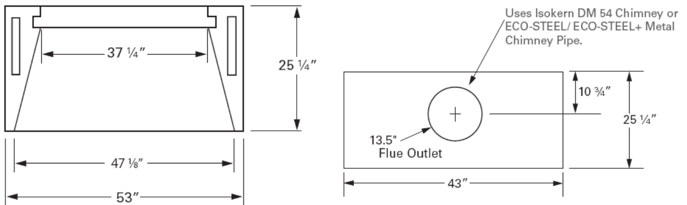
Plan View
