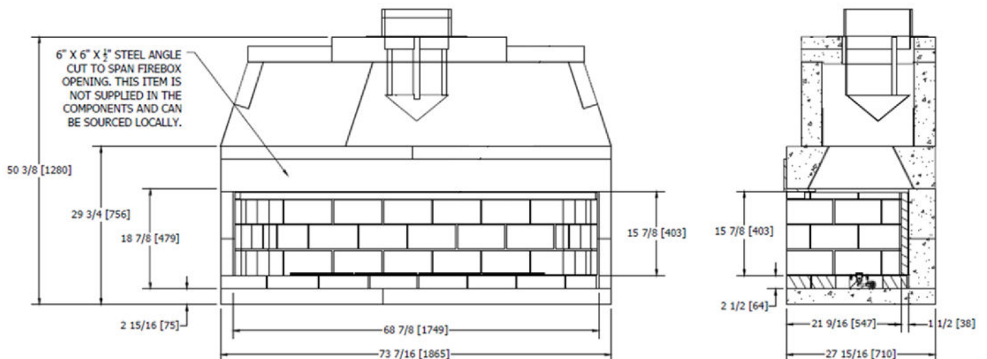
FRONT VIEW
