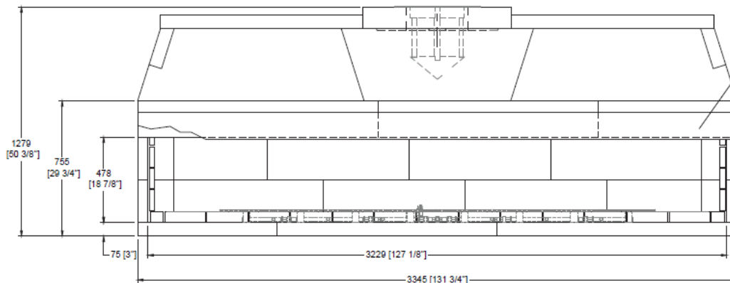
Front View
