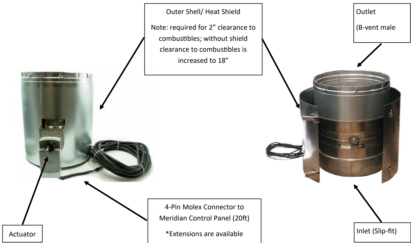
Damper Assembly
