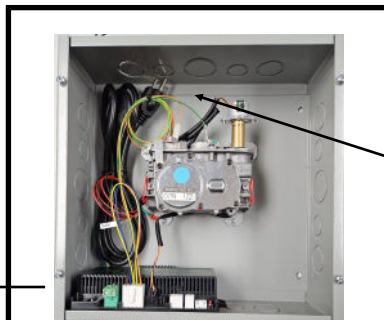
E-VKN/ E-VKP Gas Valve: 4-pin Molex to Gas Control Valve
