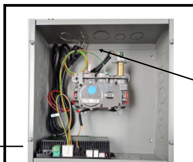
Gas Valve: 4-pin Molex to Gas Control Valve with valve wiring harness
