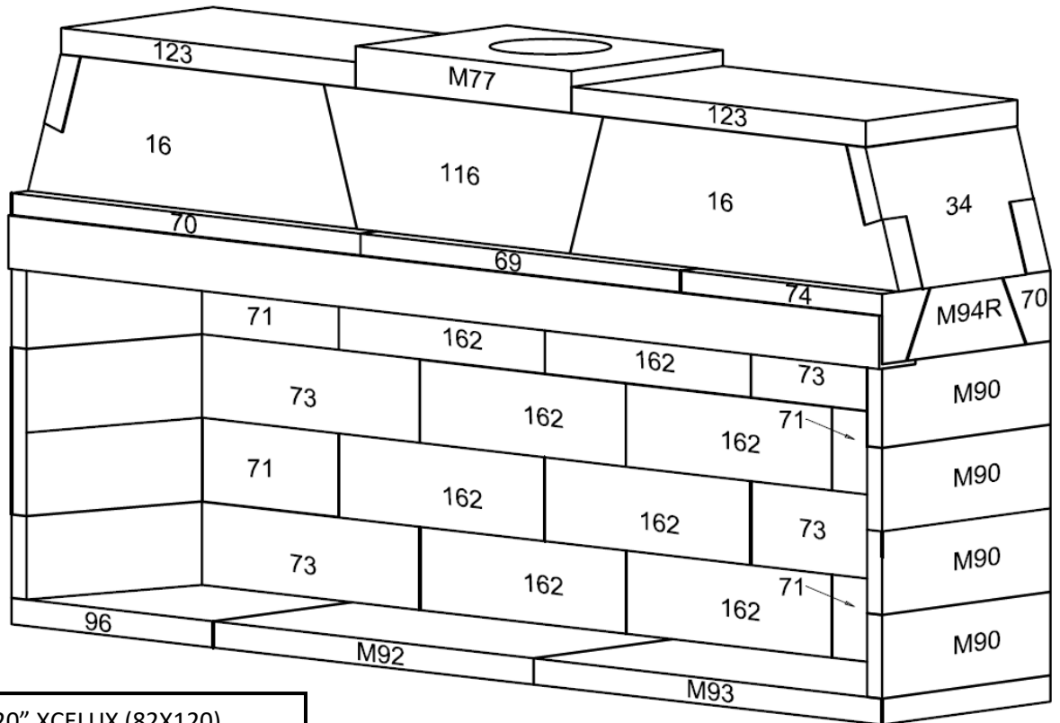
Assembled 120" XCELUX (82X120)
